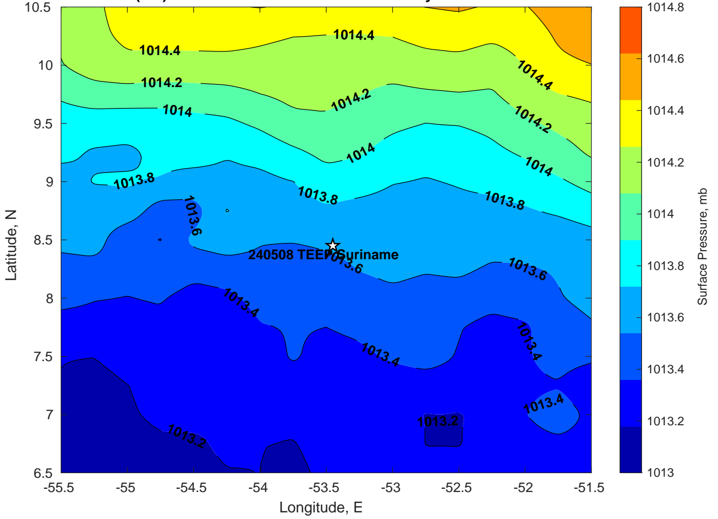
Surface Pressure (mb) for 240508 TEEP Suriname at 17-May-2024 12:00:00
