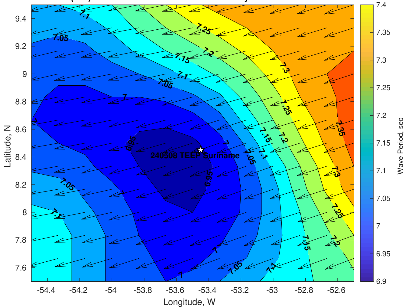
Wave Period (sec) for 240508 TEEP Suriname at 15-May-2024 18:00:00
