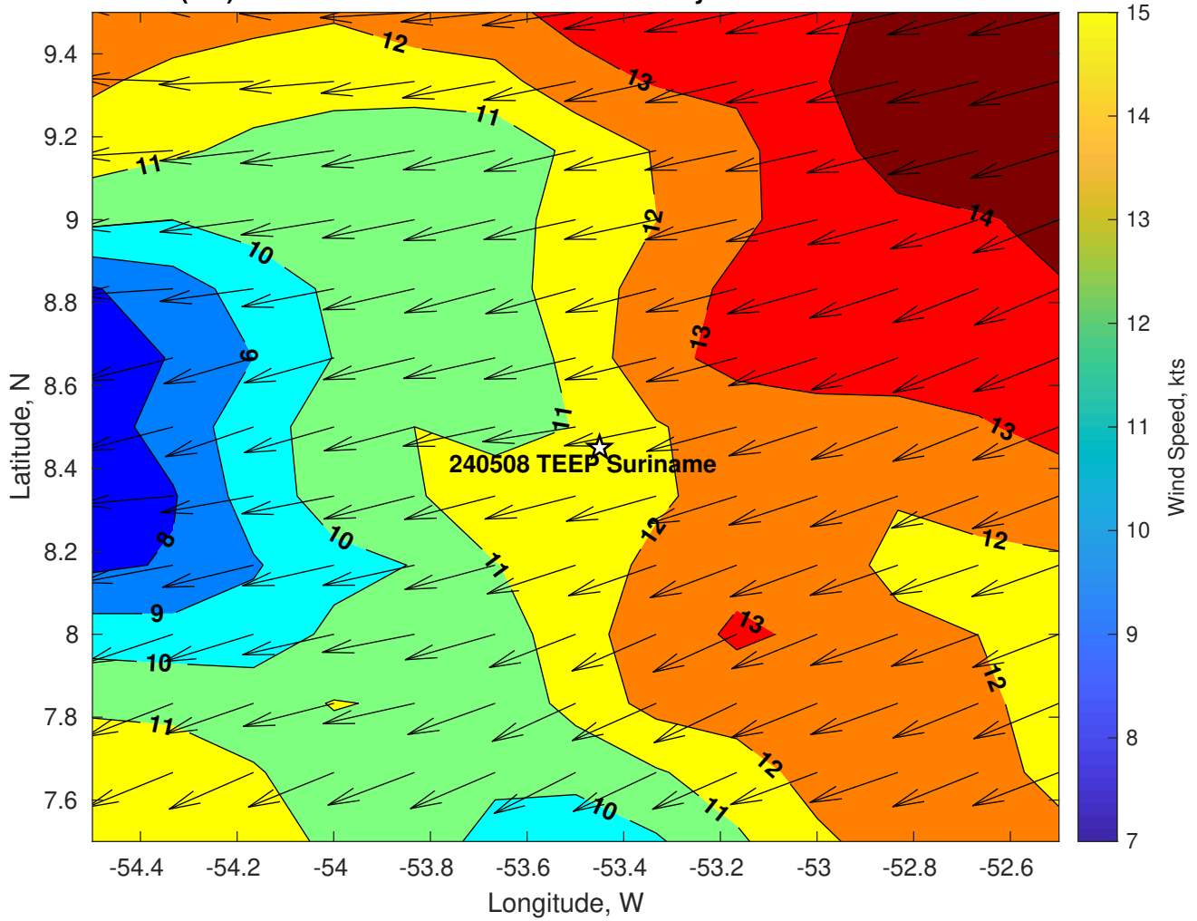
Winds (kts) for 240508 TEEP Suriname at 15-May-2024 18:00:00
