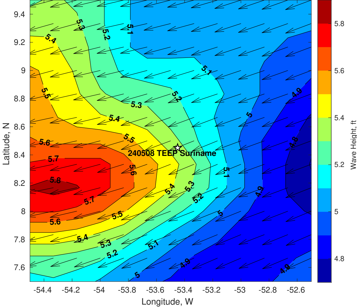
Wave Height (ft) for 240508 TEEP Suriname at 15-May-2024 18:00:00
