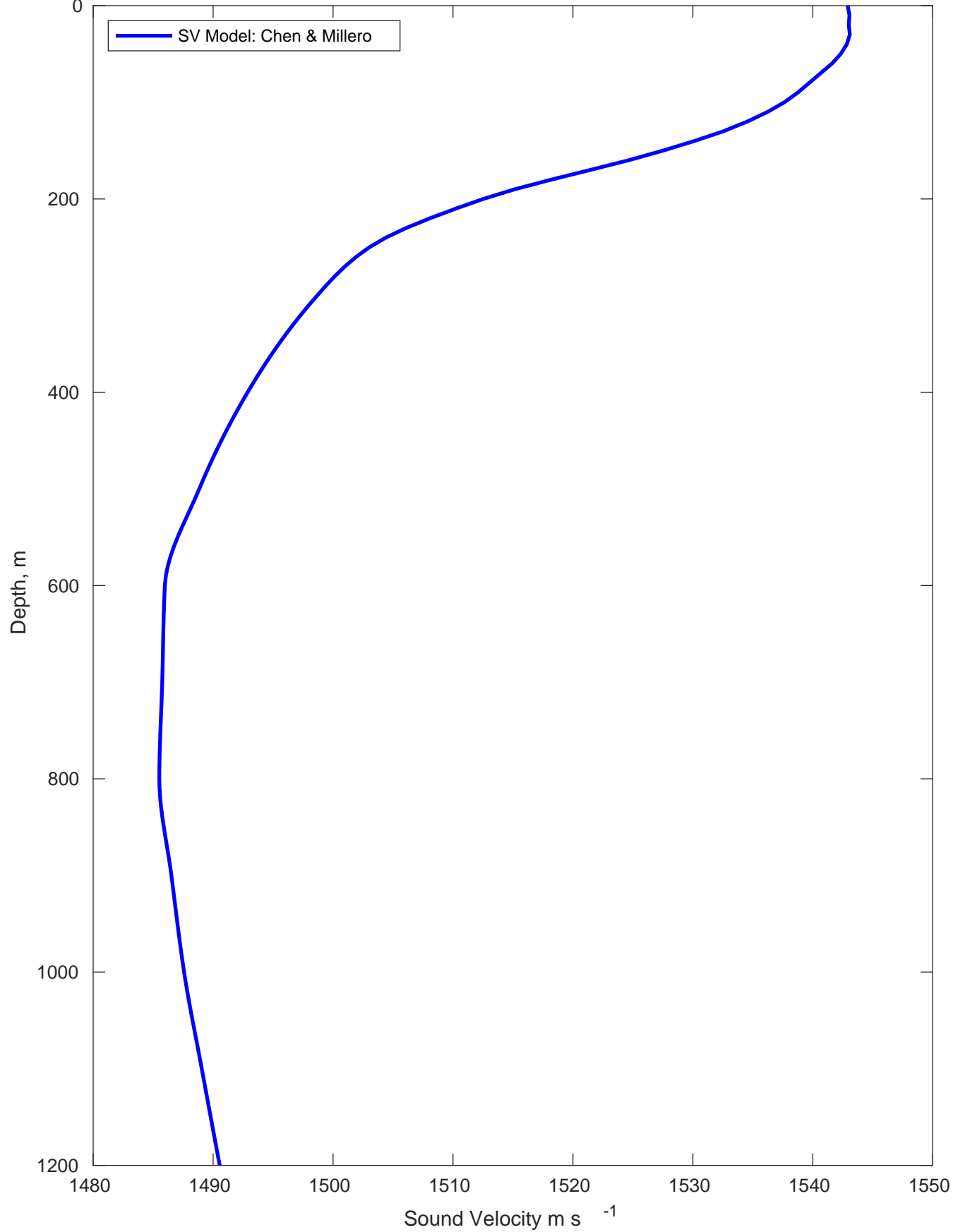
Sound Velocity Profile for 240508 TEEP Suriname on 15-May-2024 00:00:00
