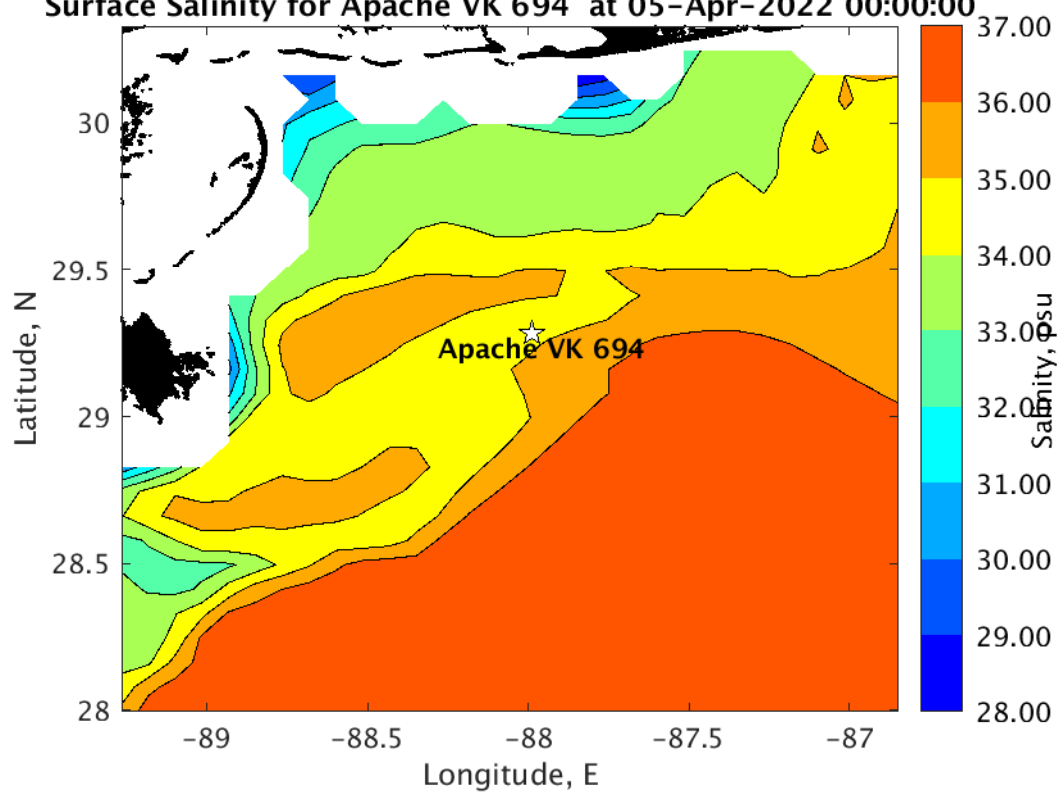
Surface Salinity for Apache VK 694 at 05-Apr-2022 00:00:00
