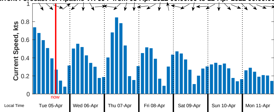
Current Forecast for Apache VK 694 from 05-Apr-2022 00:00:00 to 12-Apr-2022 00:00:00
