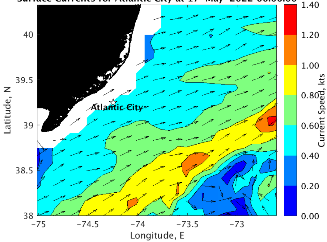
Surface Currents for Atlantic City at 17-May-2022 00:00:00
