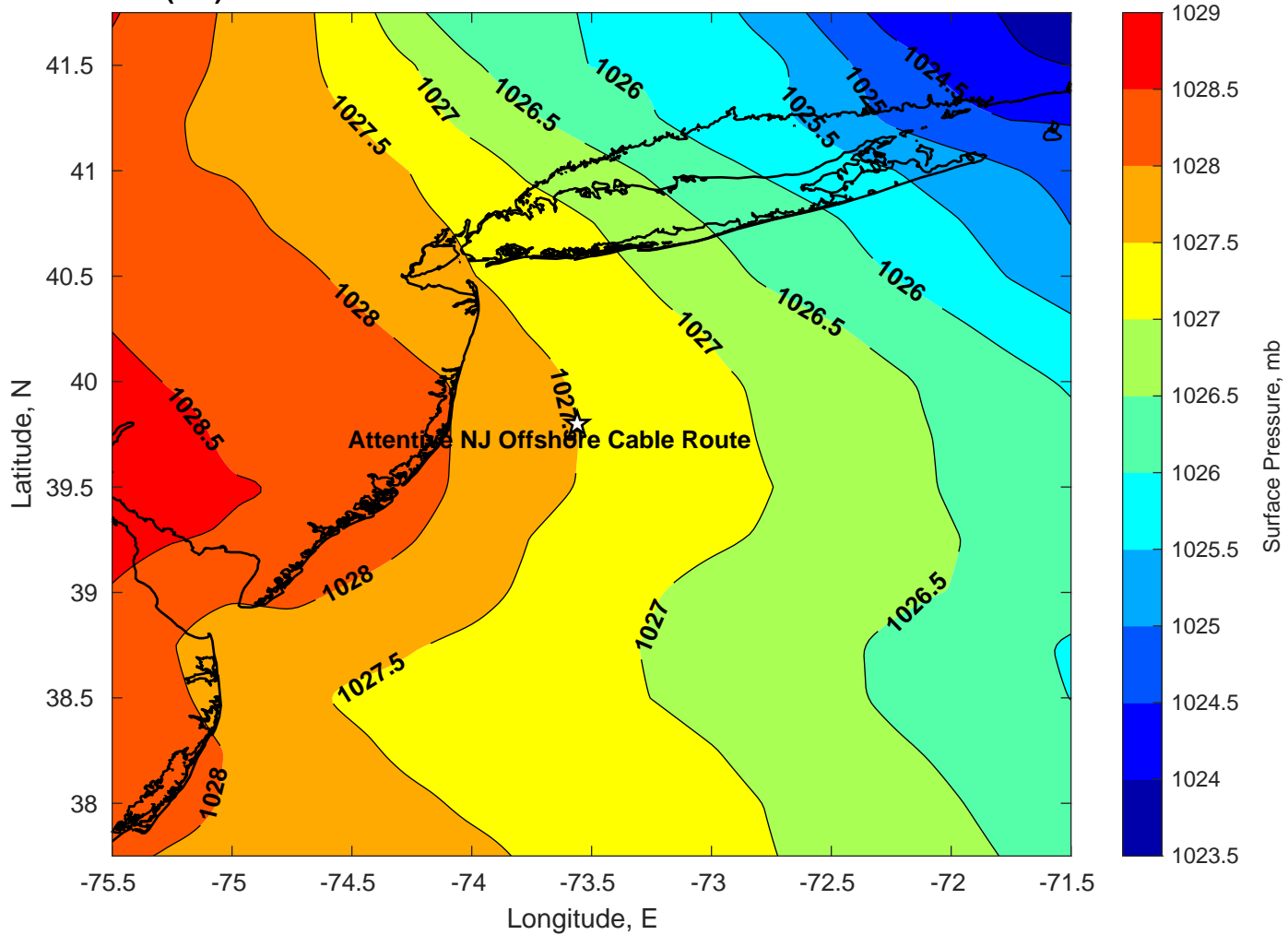
Surface Pressure (mb) for Attentive NJ Offshore Cable Route at 22-Mar-2024 06:00:00
