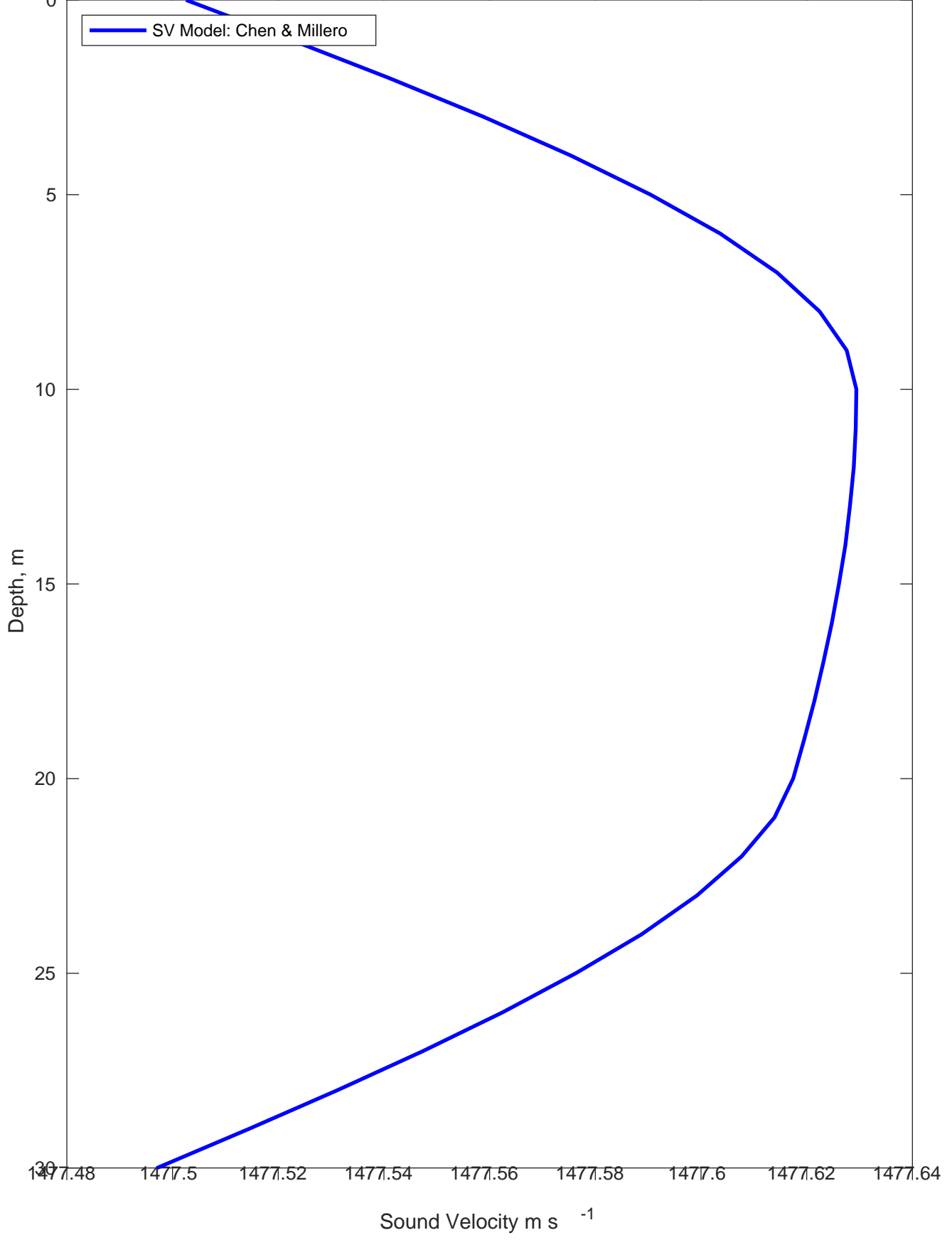
Sound Velocity Profile for Attentive NJ Offshore Cable Route on 20-Mar-2024 00:00:00
