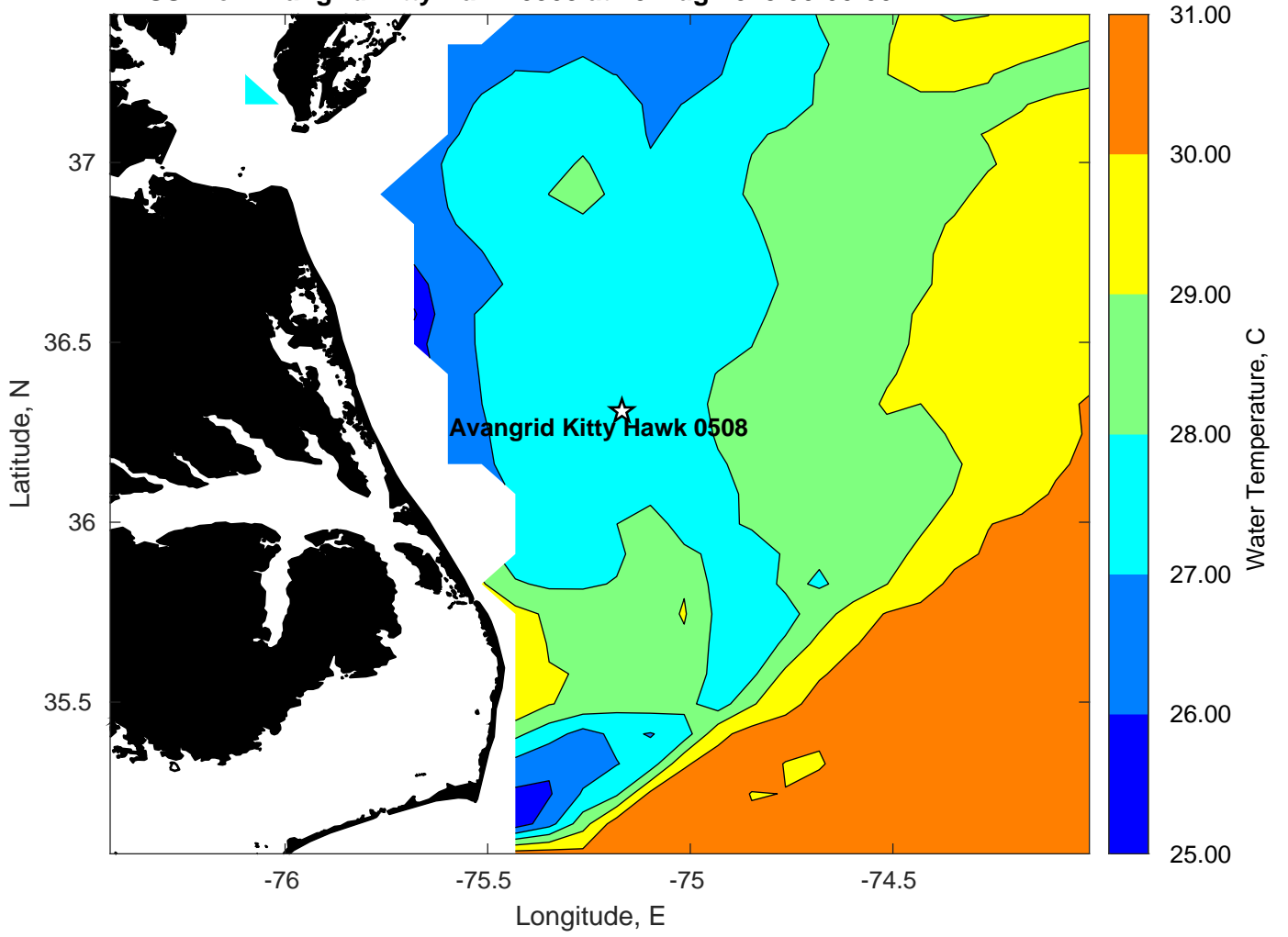
SST for Avangrid Kitty Hawk 0508 at 15-Aug-2023 00:00:00
