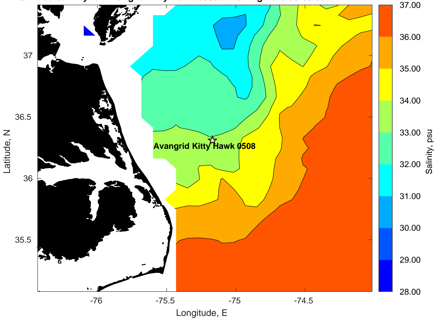
Surface Salinity for Avangrid Kitty Hawk 0508 at 15-Aug-2023 00:00:00
