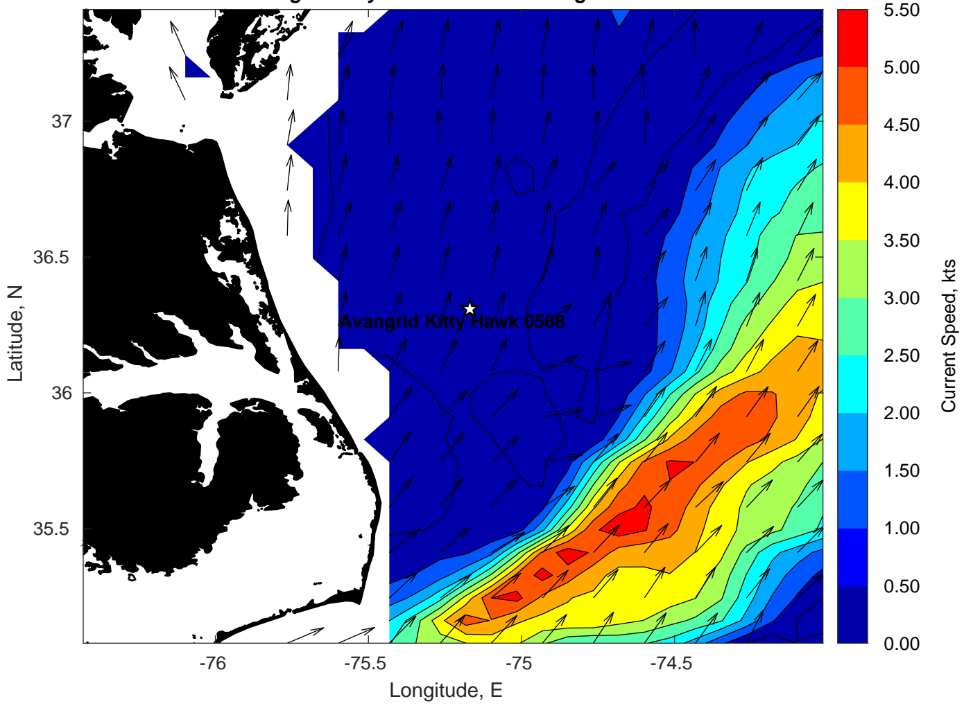
Surface Currents for Avangrid Kitty Hawk 0508 at 15-Aug-2023 00:00:00
