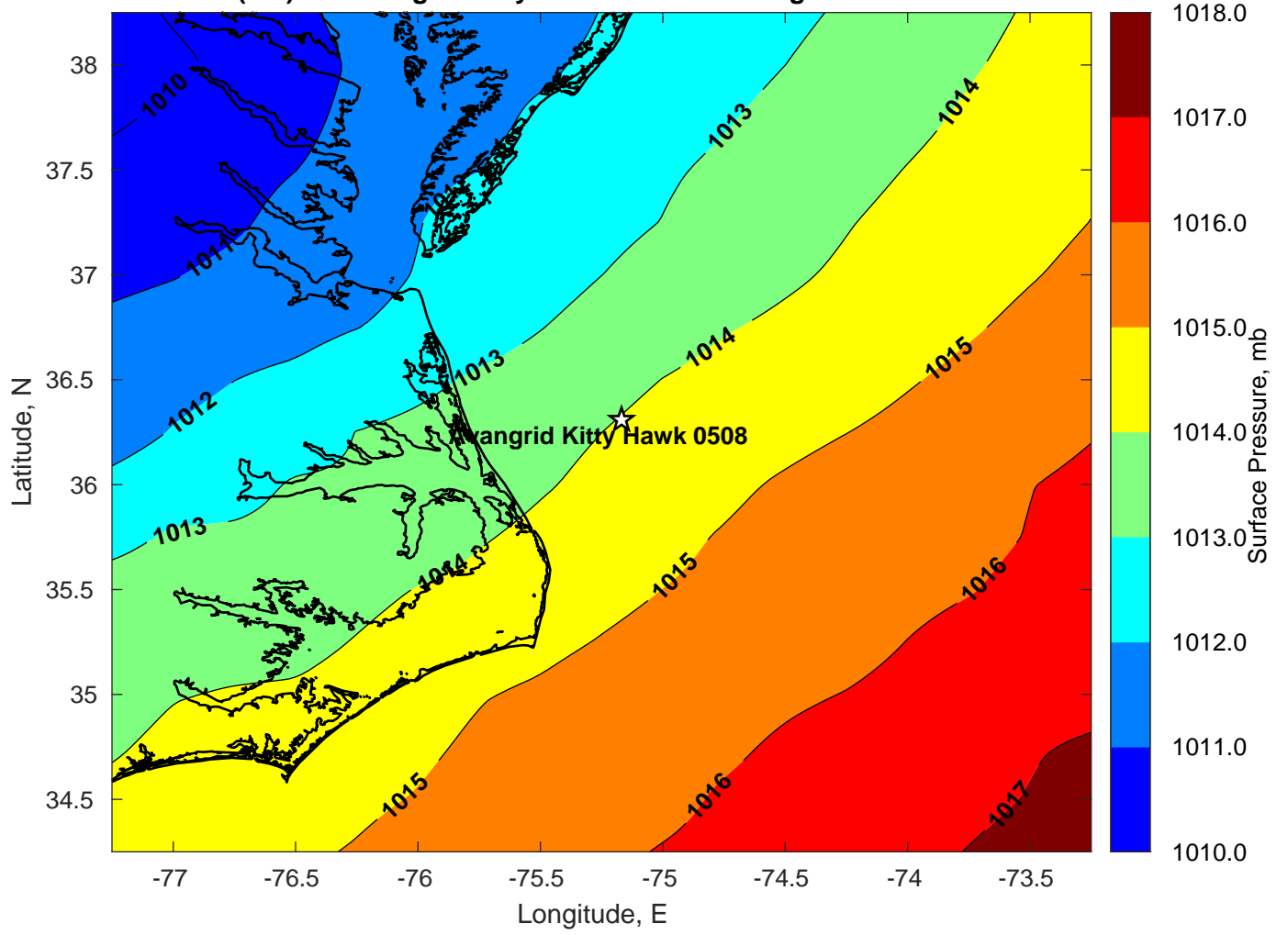
Surface Pressure (mb) for Avangrid Kitty Hawk 0508 at 17-Aug-2023 18:00:00
