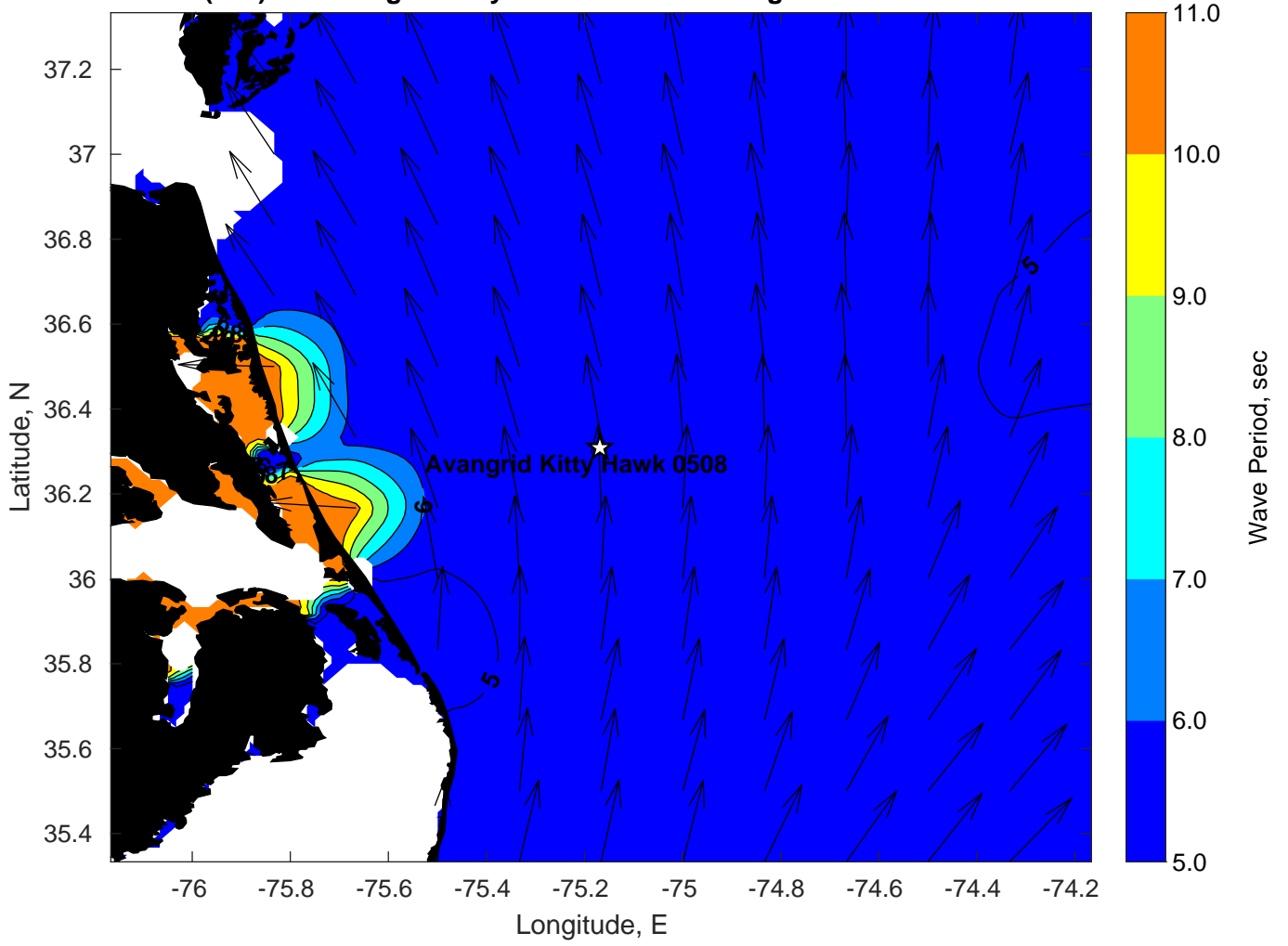
Wave Period (sec) for Avangrid Kitty Hawk 0508 at 15-Aug-2023 18:00:00
