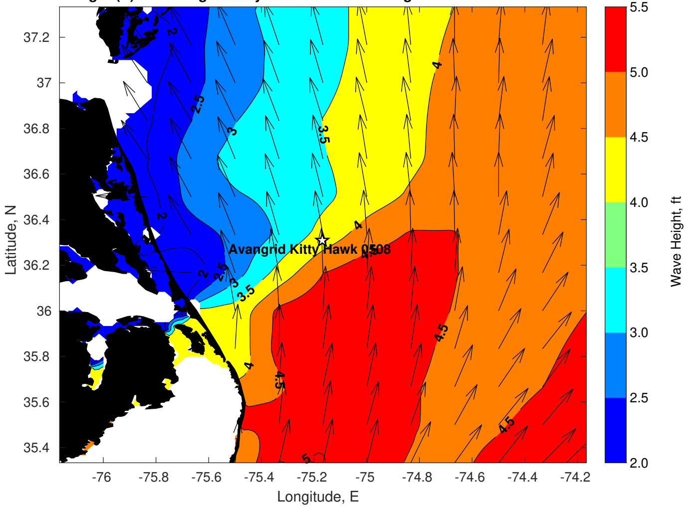
Wave Height (ft) for Avangrid Kitty Hawk 0508 at 15-Aug-2023 18:00:00
