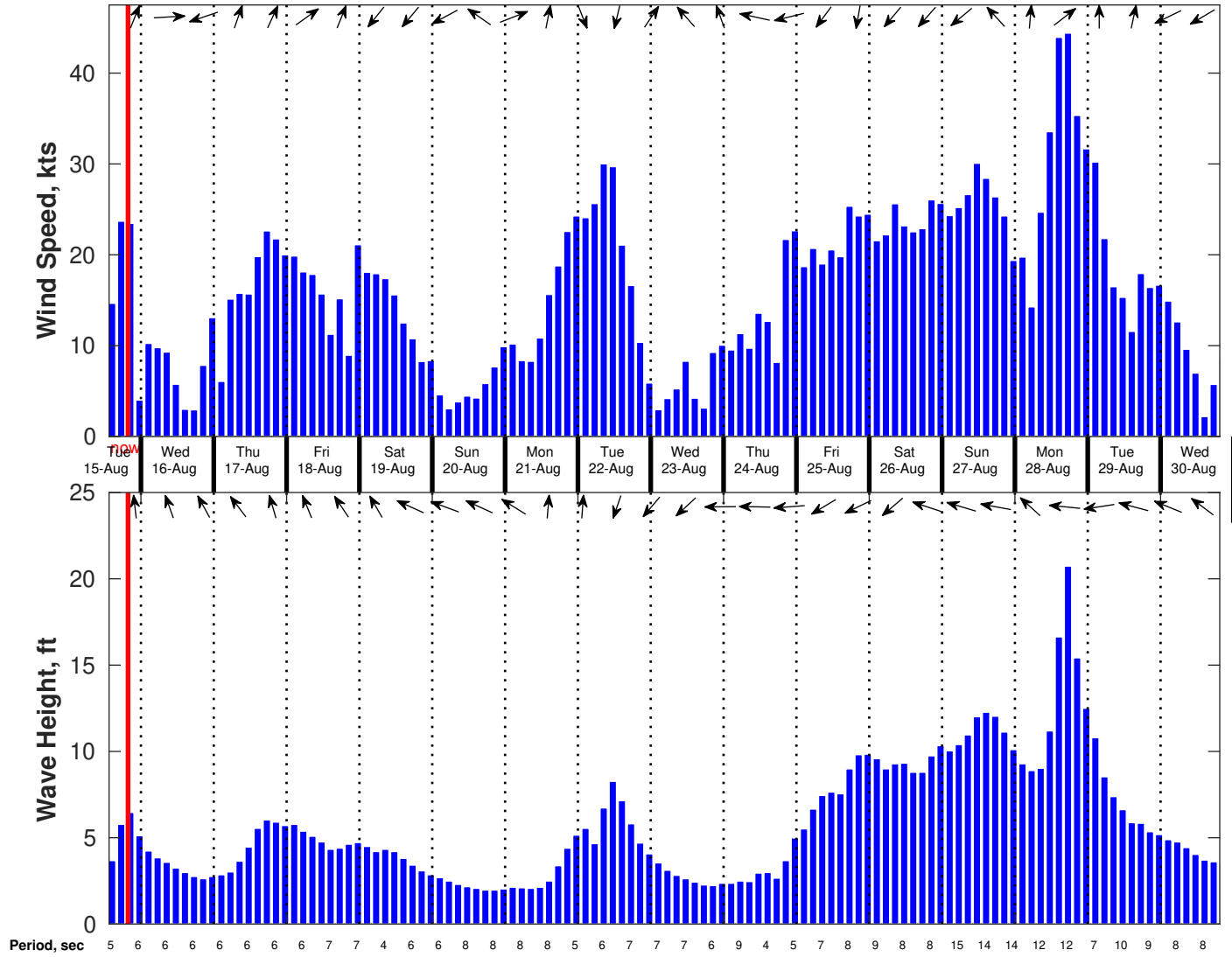
Wind & Wave Forecast for Avangrid Kitty Hawk 0508 from 15-Aug-2023 13:00:00 to 31-Aug-2023 13:00:00
