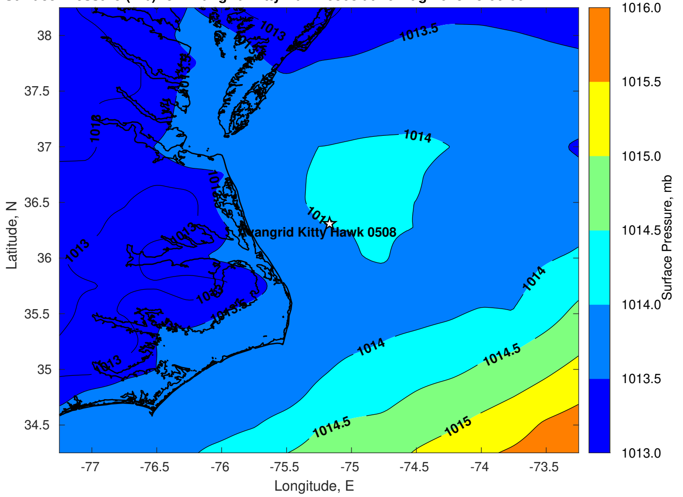
Surface Pressure (mb) for Avangrid Kitty Hawk 0508 at 16-Aug-2023 18:00:00
