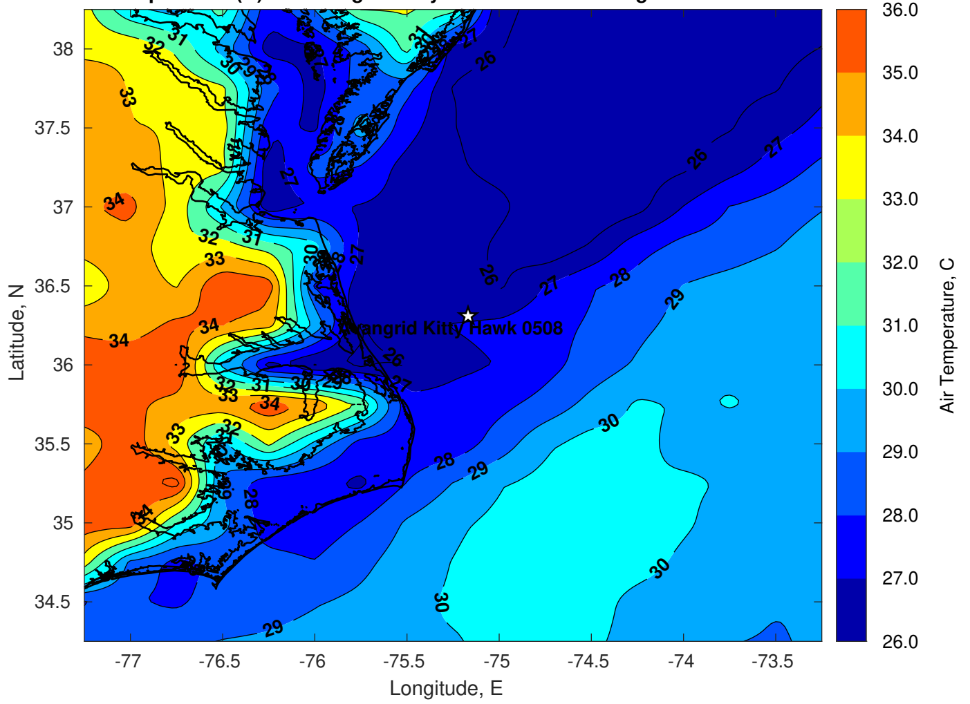
Air Temperature (C) for Avangrid Kitty Hawk 0508 at 15-Aug-2023
