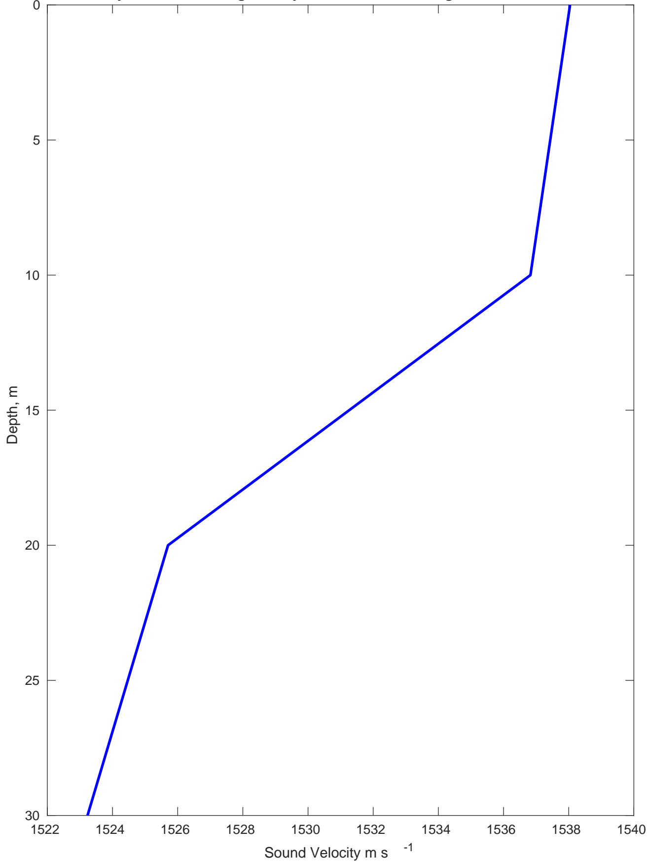
Sound Velocity Profile for Avangrid Kitty Hawk 0508 on 15-Aug-2023 00:00:00
