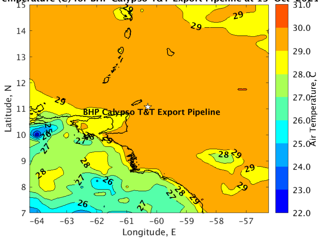
r Temperature (C) for BHP Calypso T&T Export Pipeline at 13-Oct-2021
