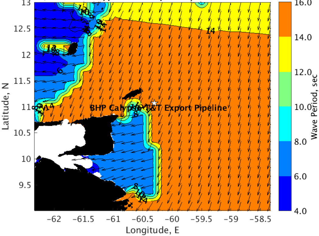
Period (sec) for BHP Calypso T&T Export Pipeline at 13-Oct-2021 12:00:00
