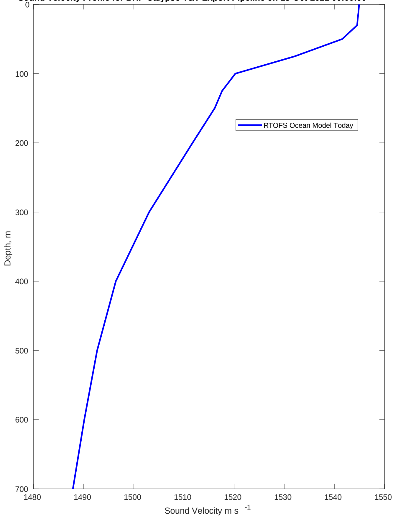
Sound Velocity Profile for BHP Calypso T&T Export Pipeline on 13-Oct-2021 00:00:00
