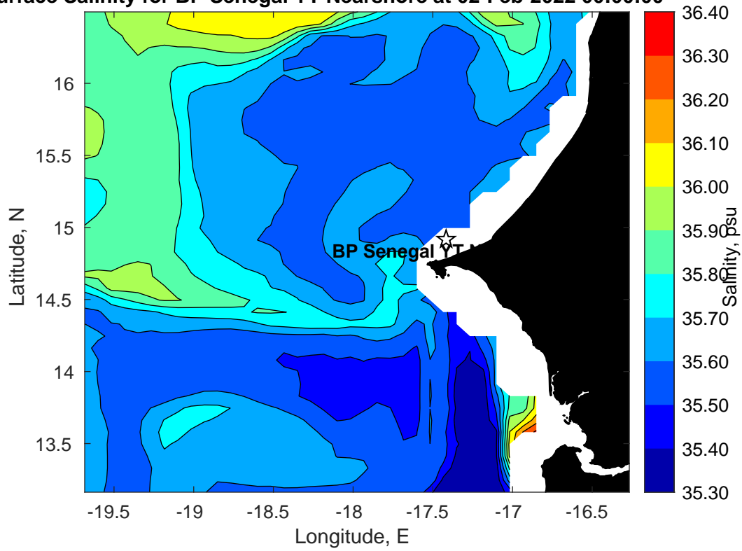
Surface Salinity for BP Senegal YT Nearshore at 02-Feb-2022 00:00:00
