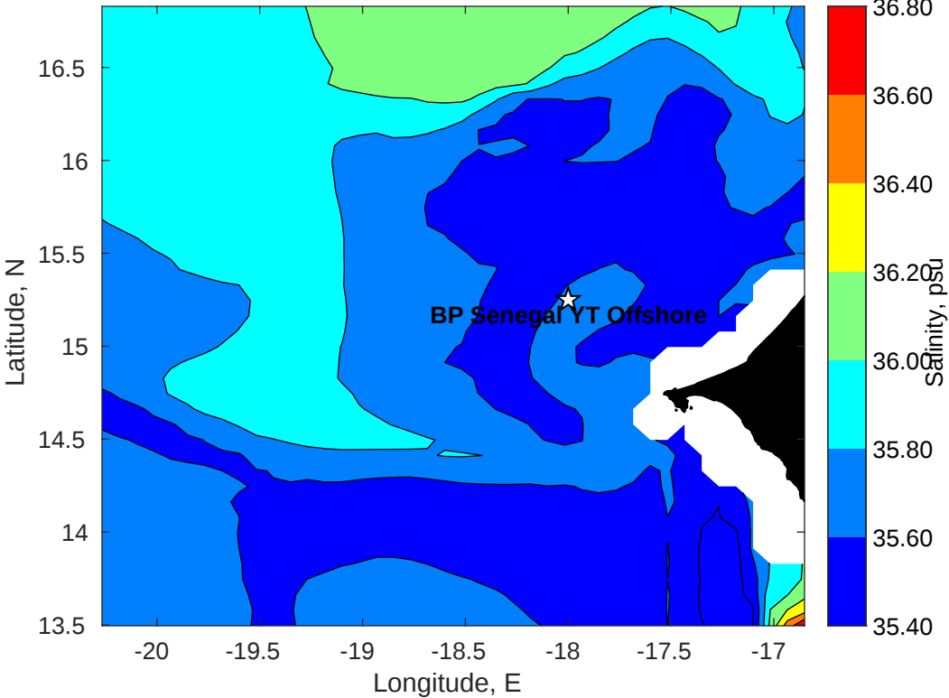
Surface Salinity for BP Senegal YT Offshore at 02-Feb-2022 00:00:00
