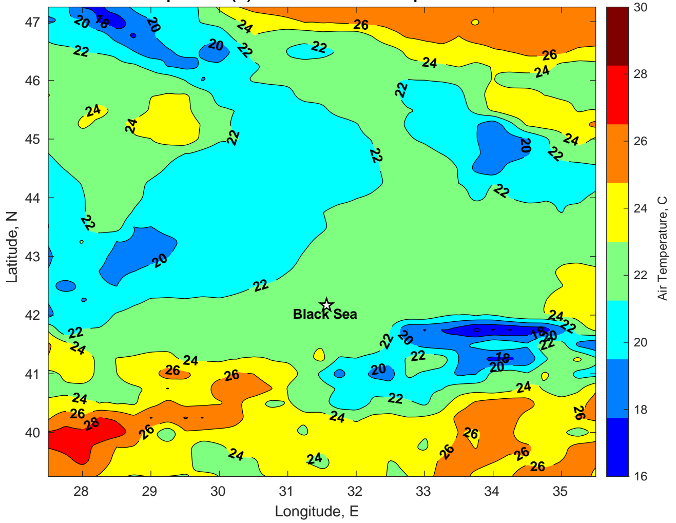
Air Temperature (C) for Black Sea at 16-Sep-2024
