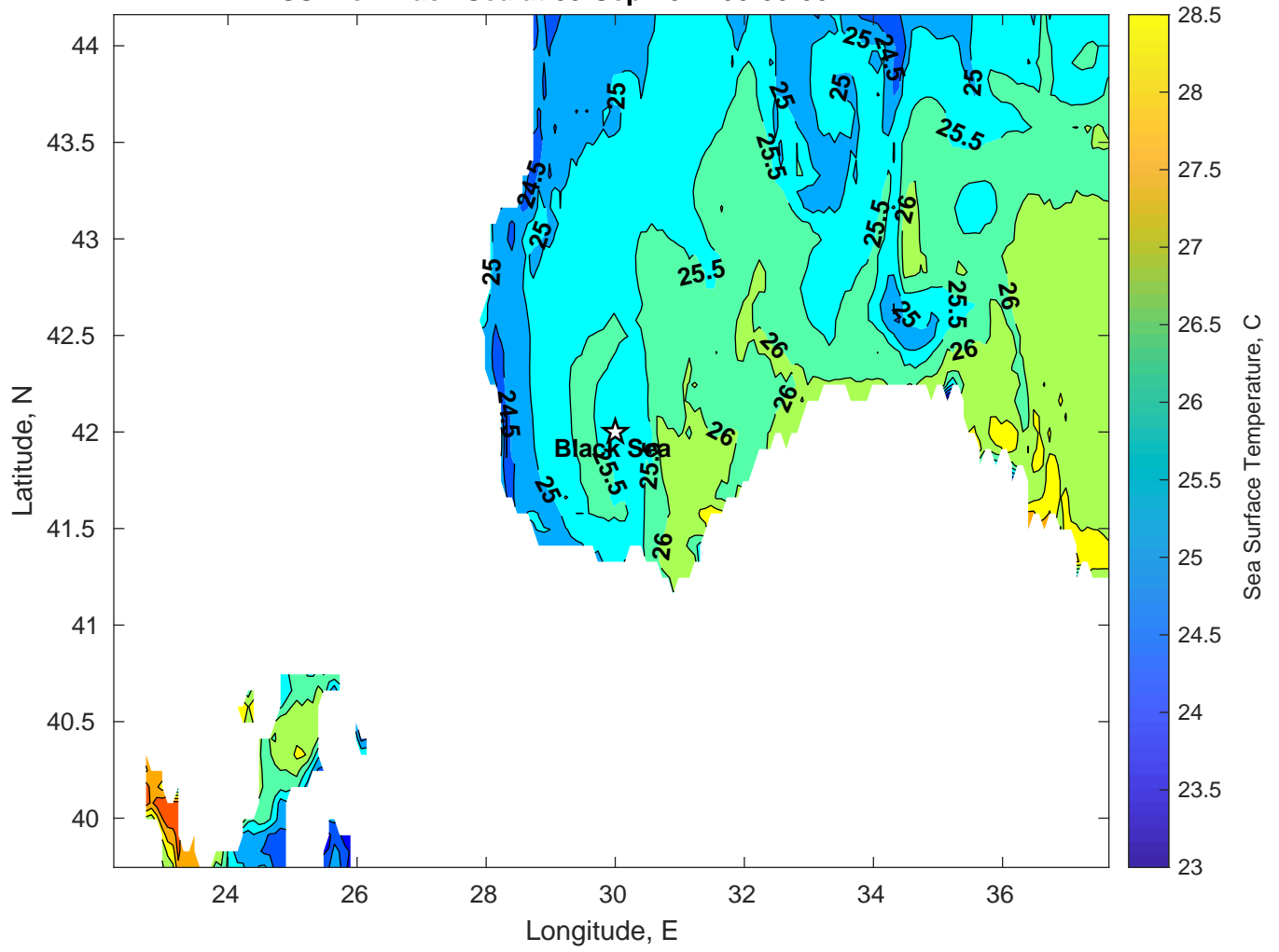
SST for Black Sea at 09-Sep-2024 00:00:00
