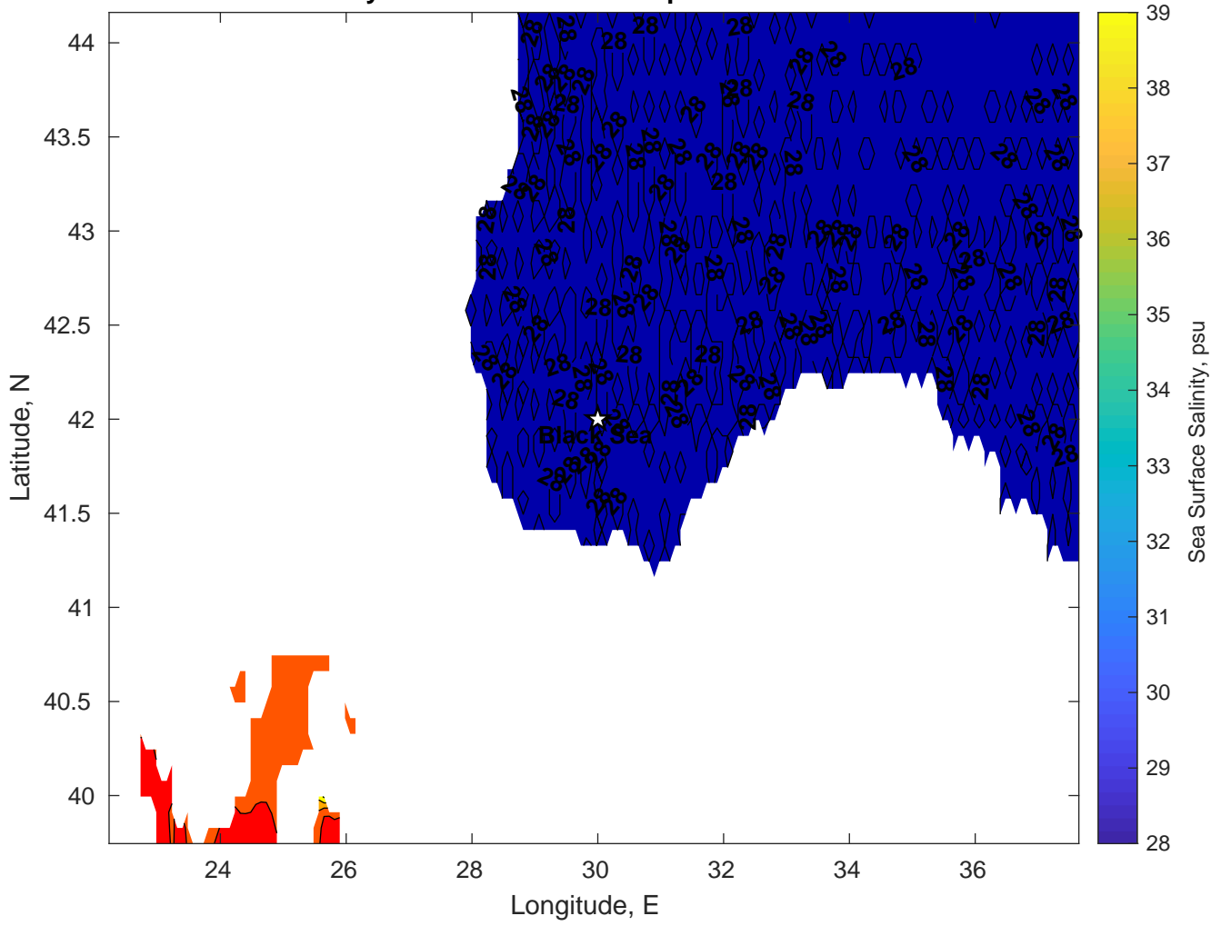
Surface Salinity for Black Sea at 09-Sep-2024 00:00:00
