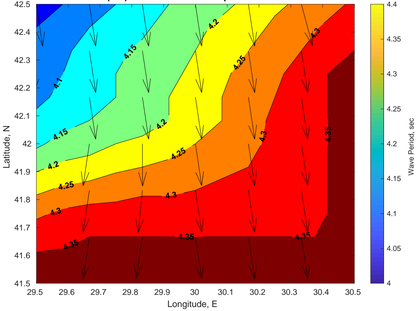
Wave Period (sec) for Black Sea at 16-Sep-2024 18:00:00
