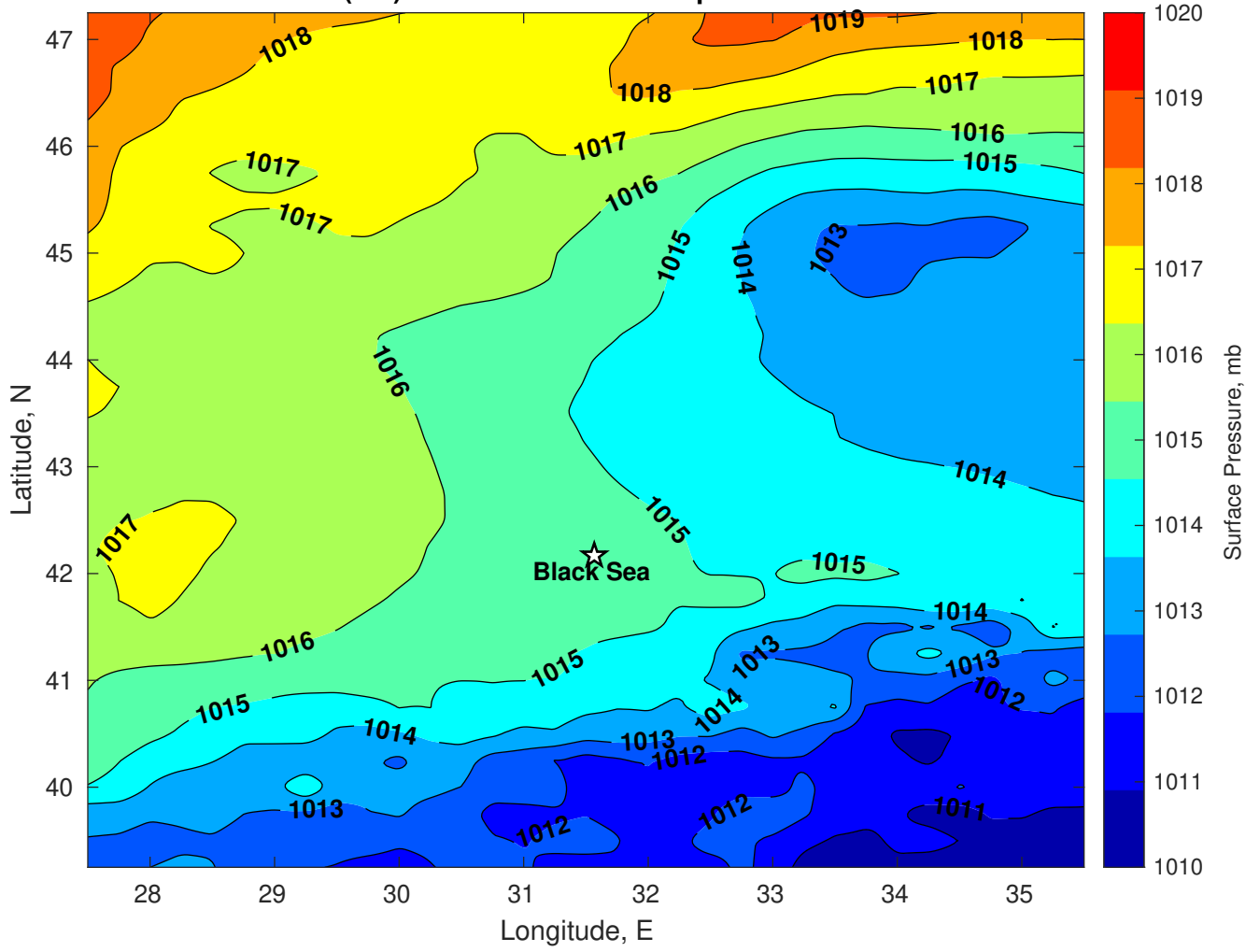
Surface Pressure (mb) for Black Sea at 17-Sep-2024 12:00:00
