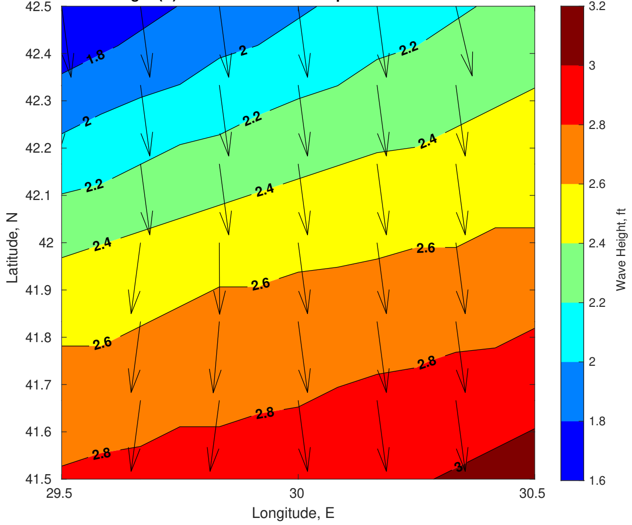
Wave Height (ft) for Black Sea at 16-Sep-2024 18:00:00
