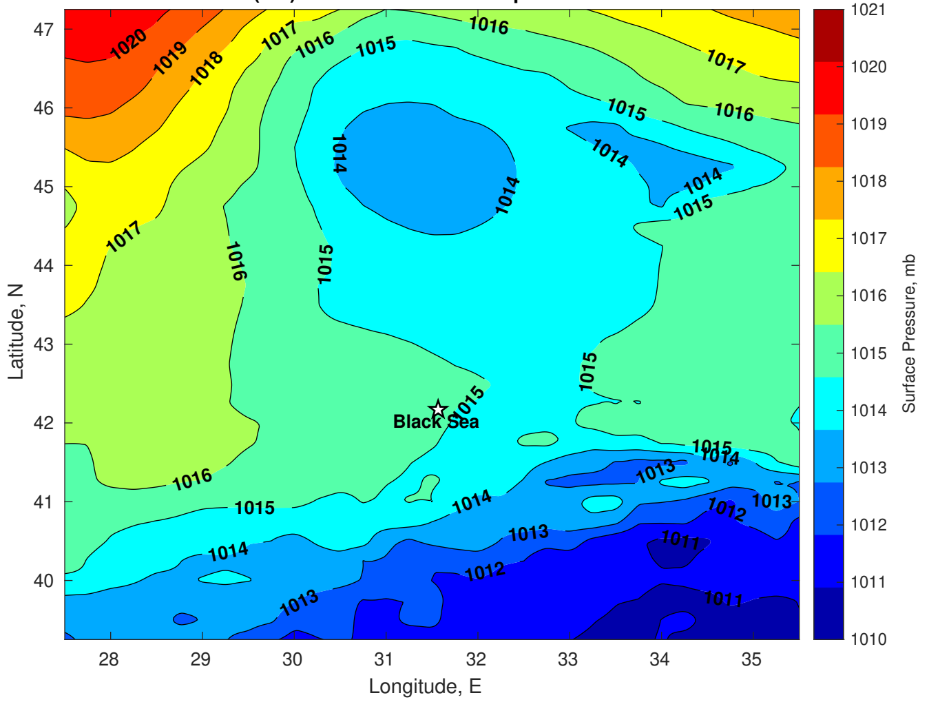
Surface Pressure (mb) for Black Sea at 18-Sep-2024 12:00:00
