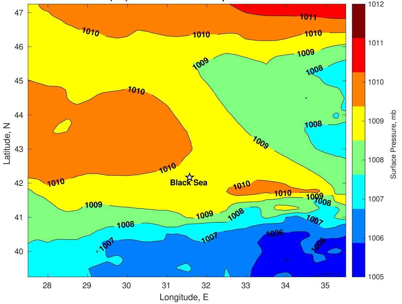
Surface Pressure (mb) for Black Sea at 16-Sep-2024 12:00:00
