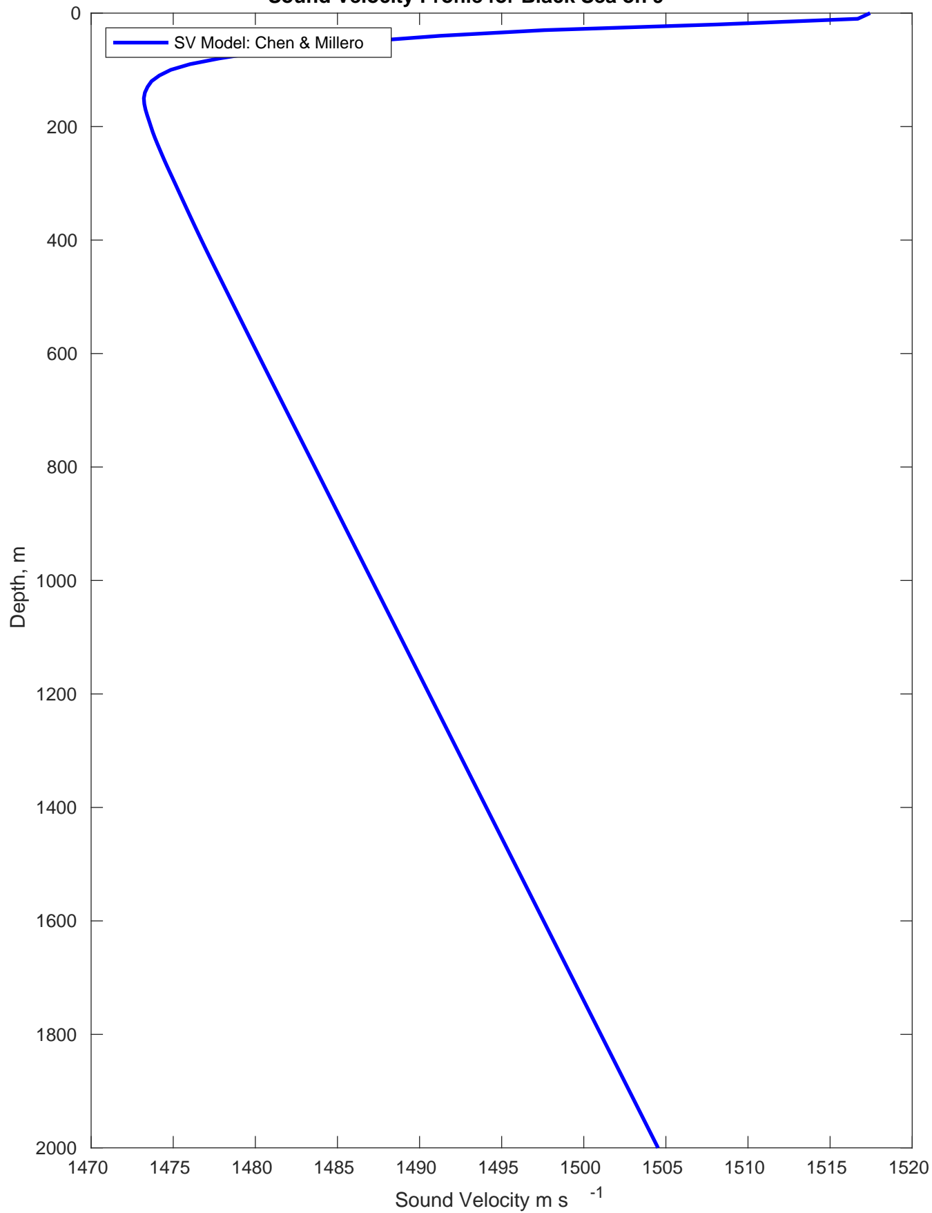
Sound Velocity Profile for Black Sea on 9
