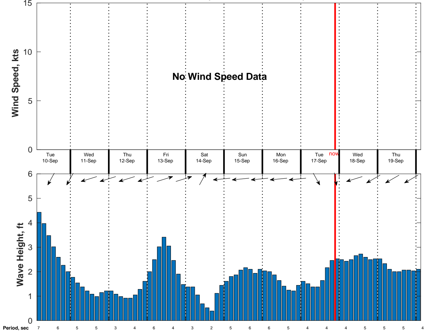
Wind & Wave Forecast for Black Sea from 09-Sep-2024 03:00:00 to 19-Sep-2024 03:00:00
