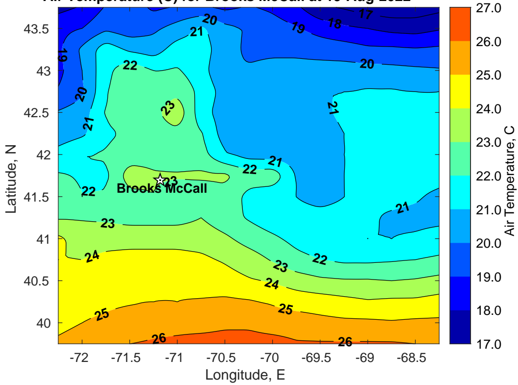
Air Temperature (C) for Brooks McCall at 19-Aug-2022
