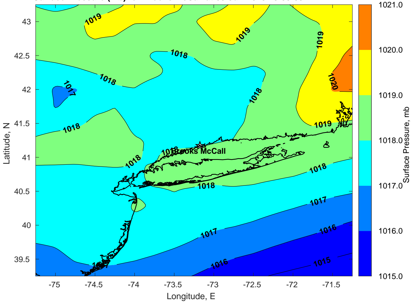
Surface Pressure (mb) for Brooks McCall at 03-Jun-2023 18:00:00
