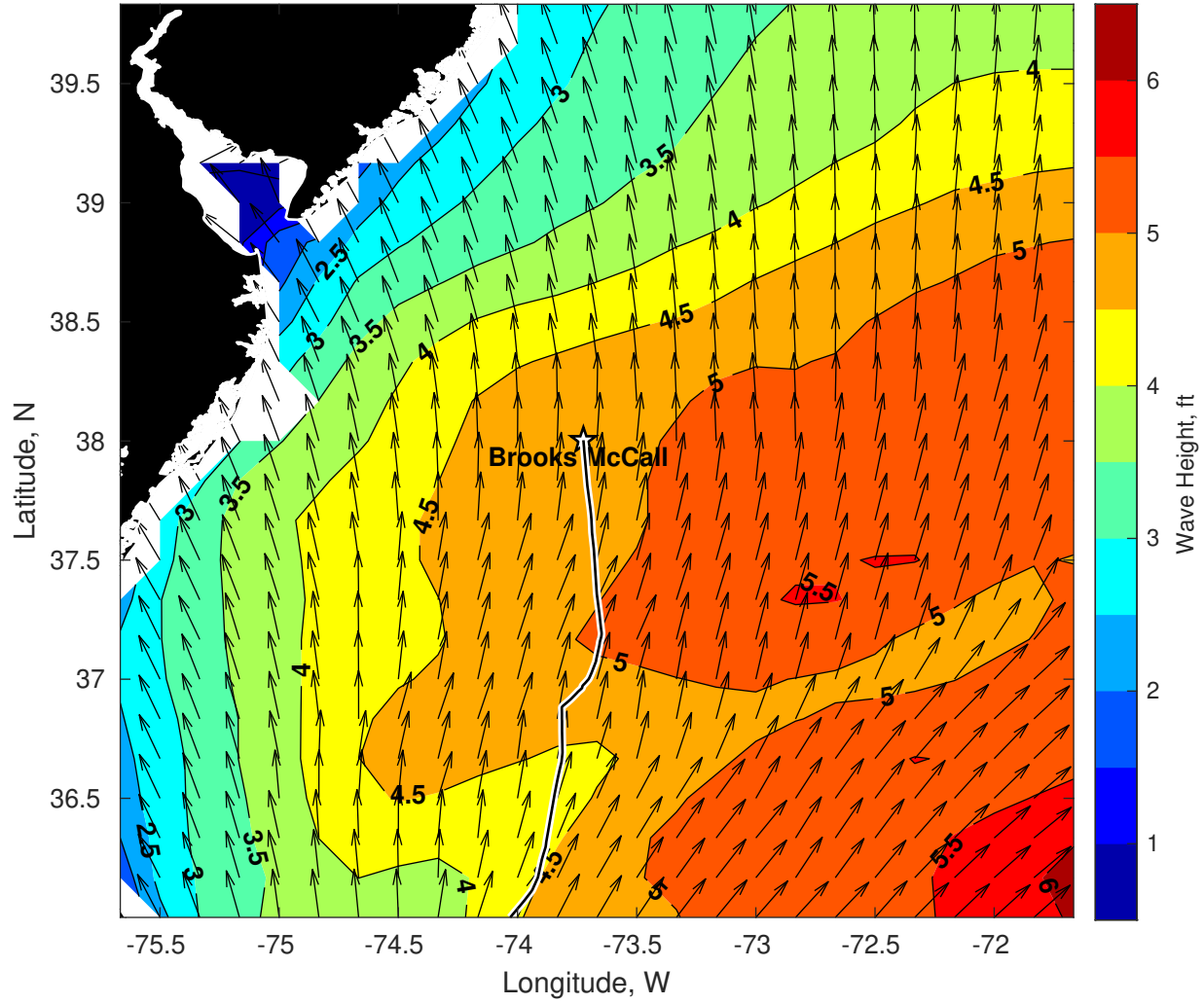
Wave Height (ft) for Brooks McCall at 25-Jul-2024 12:00:00
