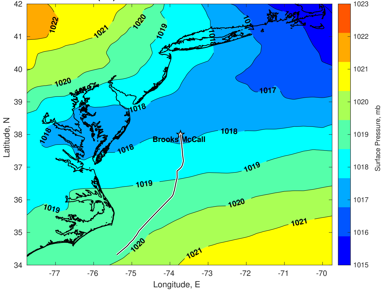
Surface Pressure (mb) for Brooks McCall at 26-Jul-2024 06:00:00
