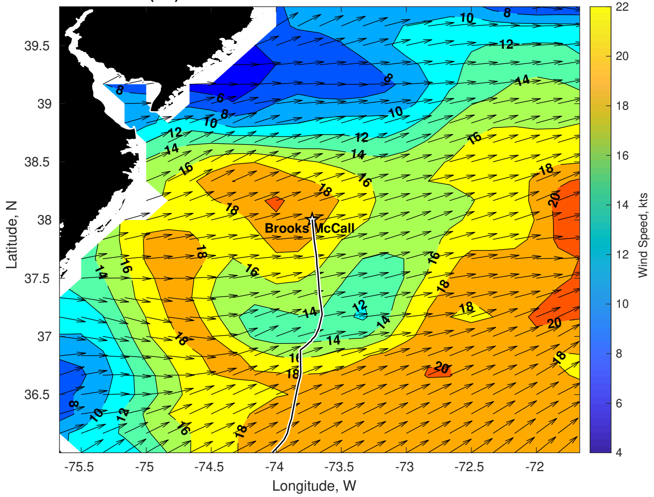
Winds (kts) for Brooks McCall at 25-Jul-2024 12:00:00
