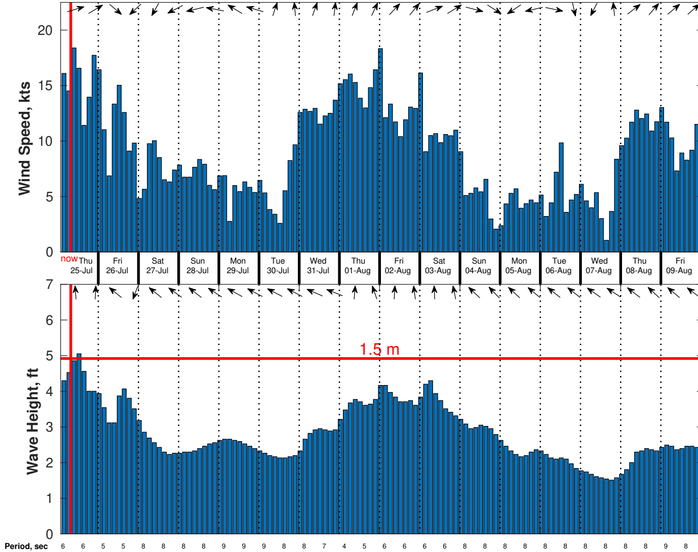
Wind & Wave Forecast for Brooks McCall from 25-Jul-2024 02:00:00 to 10-Aug-2024 02:00:00
