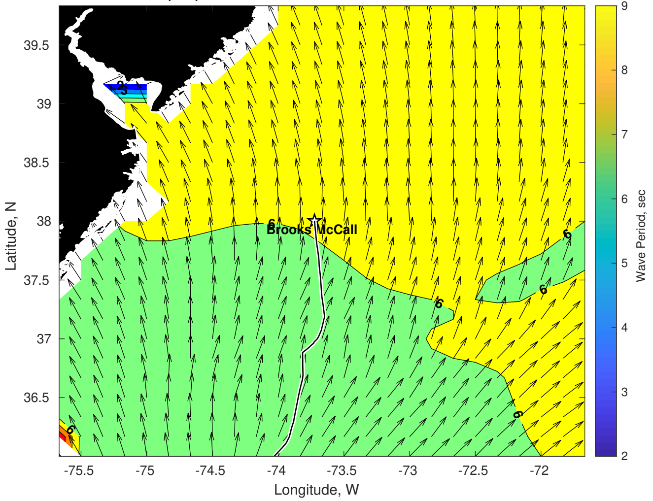
Wave Period (sec) for Brooks McCall at 25-Jul-2024 12:00:00
