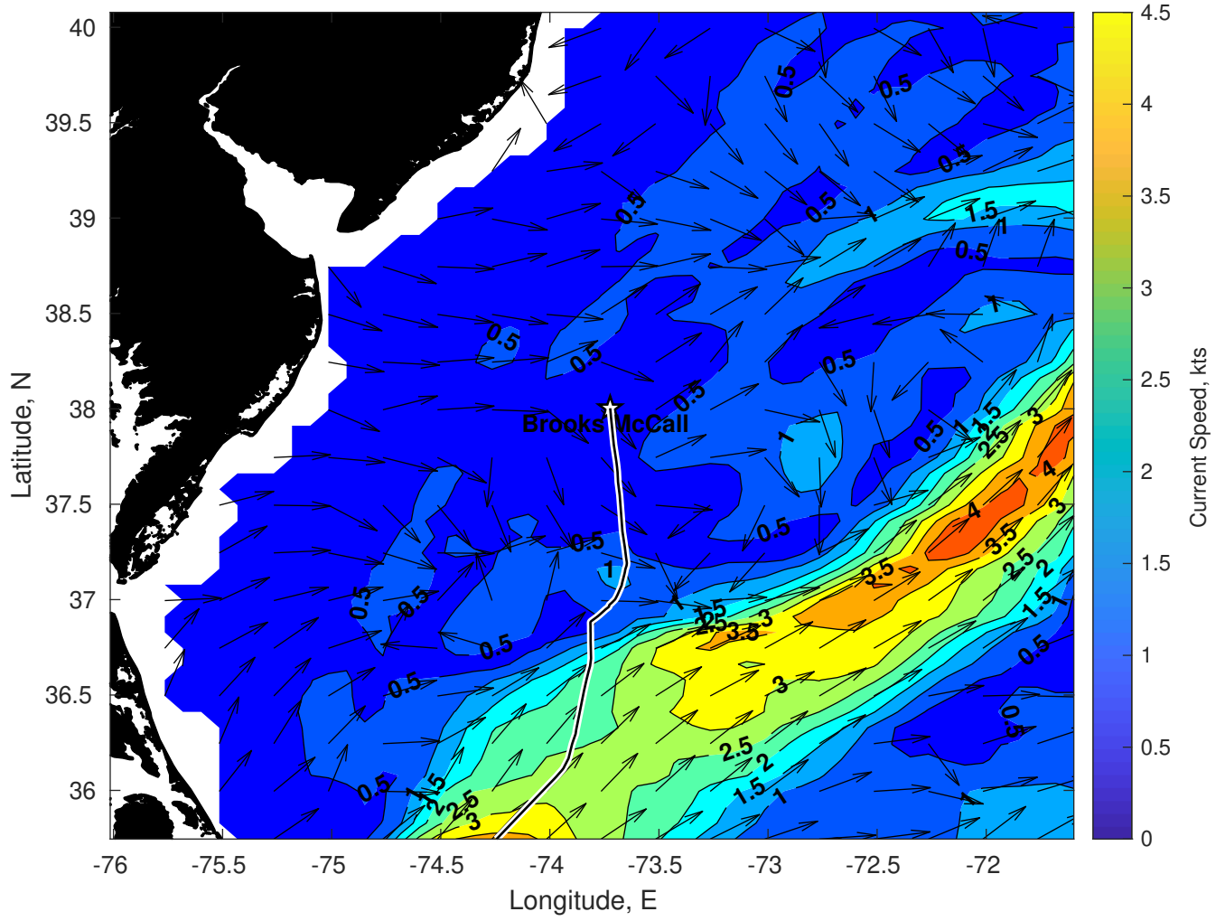
Surface Currents for Brooks McCall at 25-Jul-2024 00:00:00
