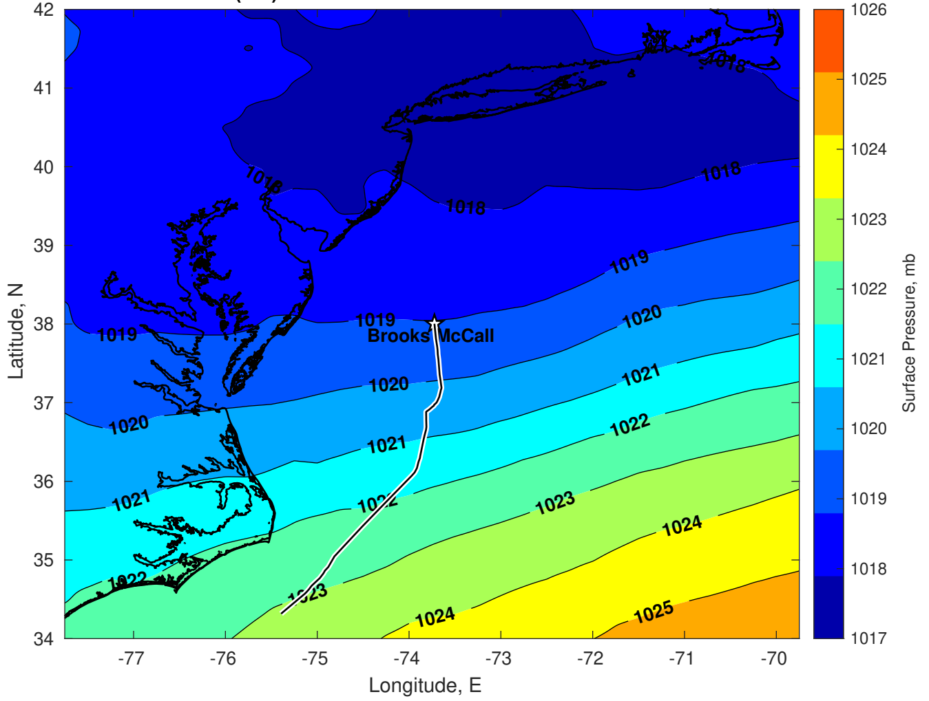
Surface Pressure (mb) for Brooks McCall at 25-Jul-2024 06:00:00
