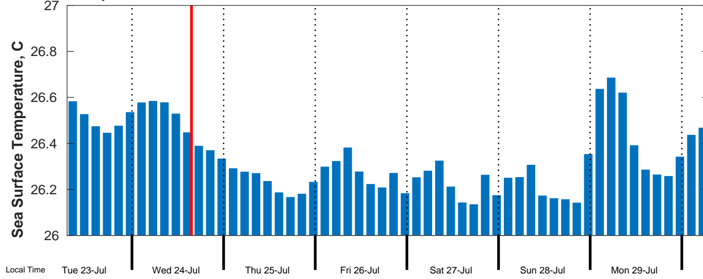
Sea Surface Temperature Forecast for Brooks McCall from 24-Jul-2024 00:00:00 to 31-Jul-2024 00:00:00
