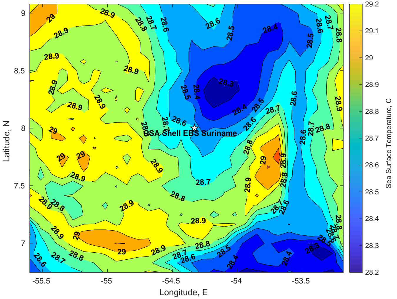
SST for CSA Shell EBS Suriname at 18-Jun-2024 00:00:00
