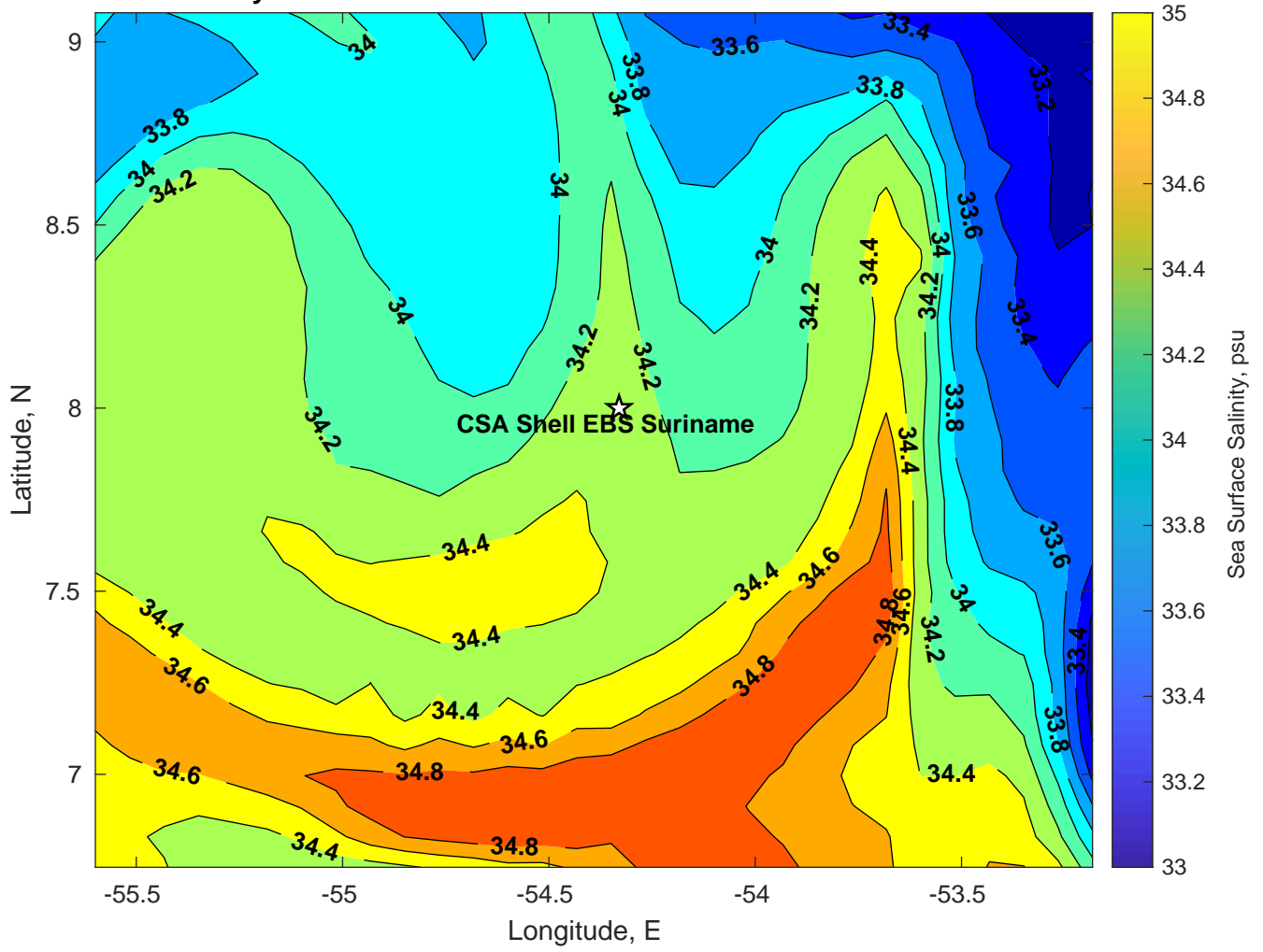
Surface Salinity for CSA Shell EBS Suriname at 18-Jun-2024 00:00:00
