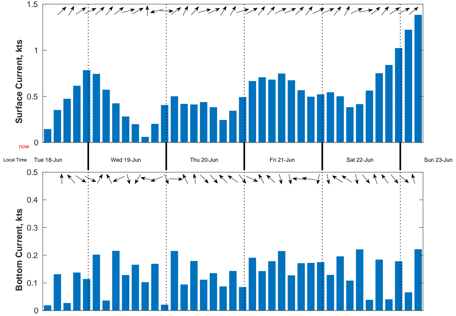
Surface Current Forecast for CSA Shell EBS Suriname from 19-Jun-2024 03:00:00 to 24-Jun-2024 00:00:00
