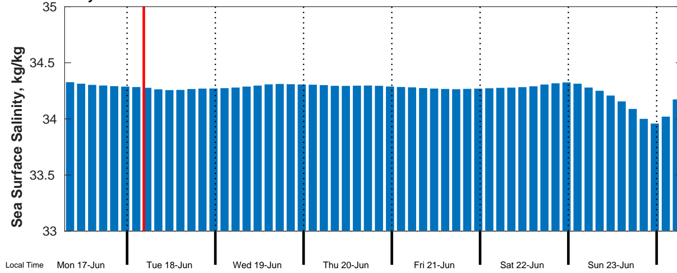
Sea Surface Salinity Forecast for CSA Shell EBS Suriname from 18-Jun-2024 00:00:00 to 25-Jun-2024 00:00:00
