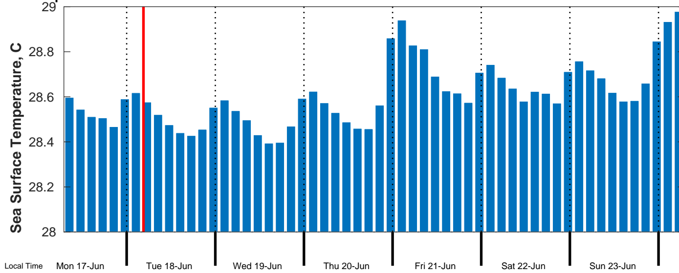
Sea Surface Temperature Forecast for CSA Shell EBS Suriname from 18-Jun-2024 00:00:00 to 25-Jun-2024 00:00:00
