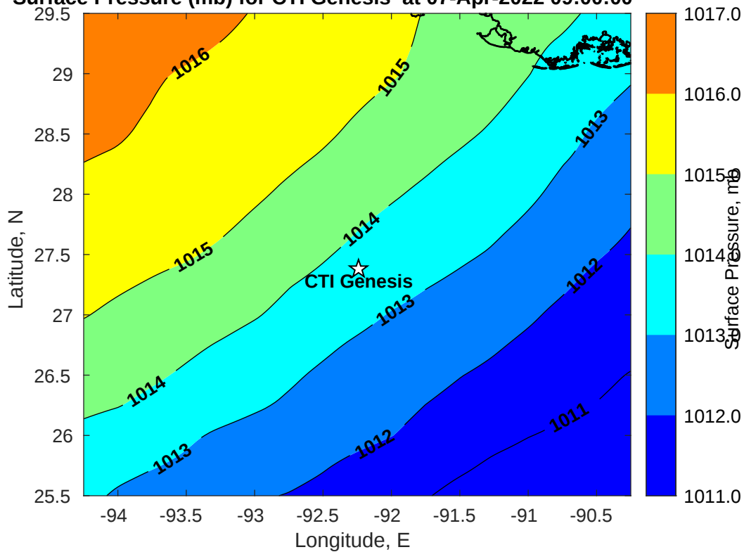
Surface Pressure (mb) for CTI Genesis at 07-Apr-2022 09:00:00
