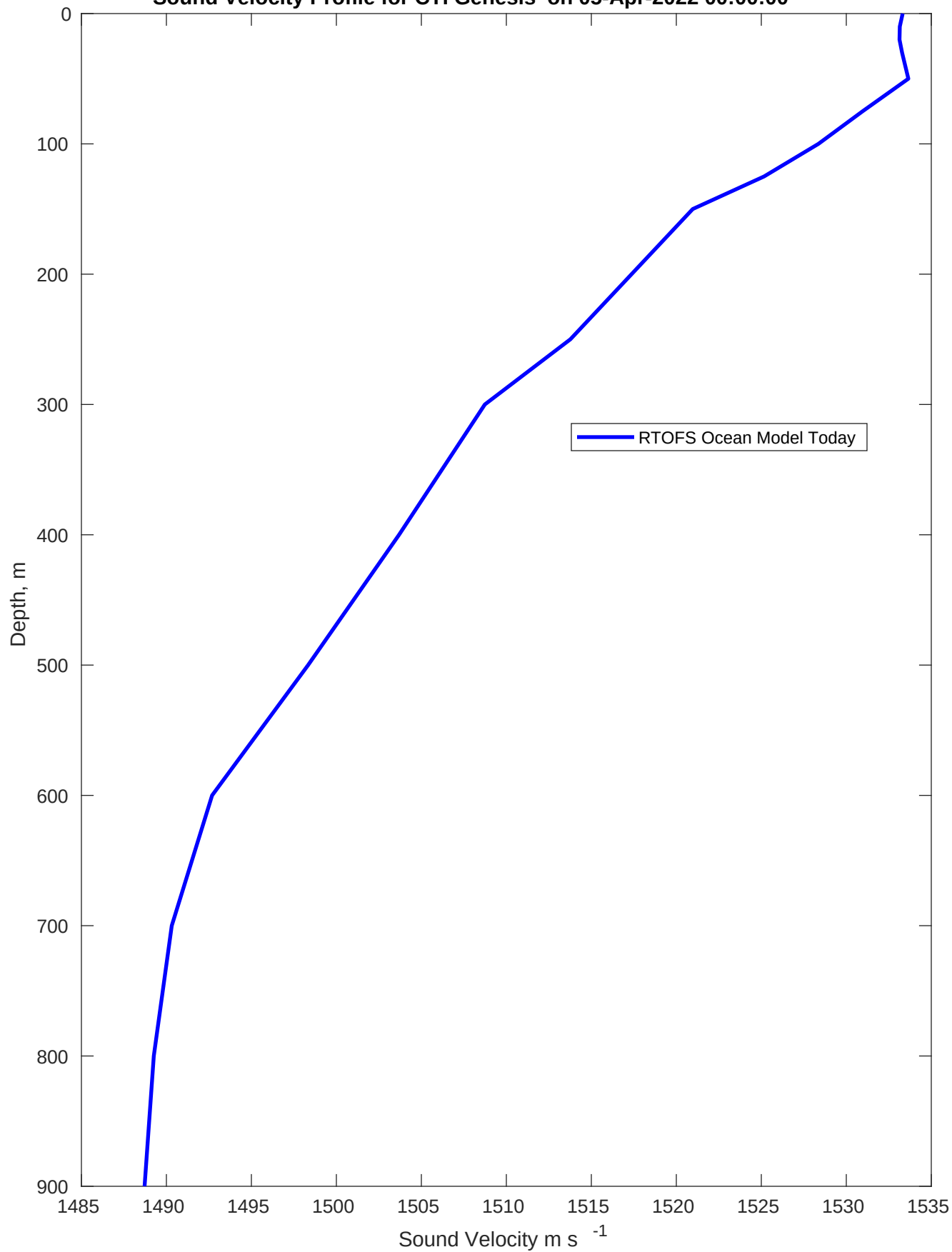
Sound Velocity Profile for CTI Genesis on 05-Apr-2022 00:00:00
