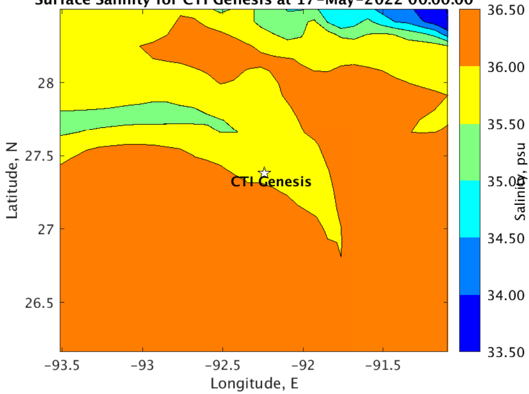
Surface Salinity for CTI Genesis at 17-May-2022 00:00:00
