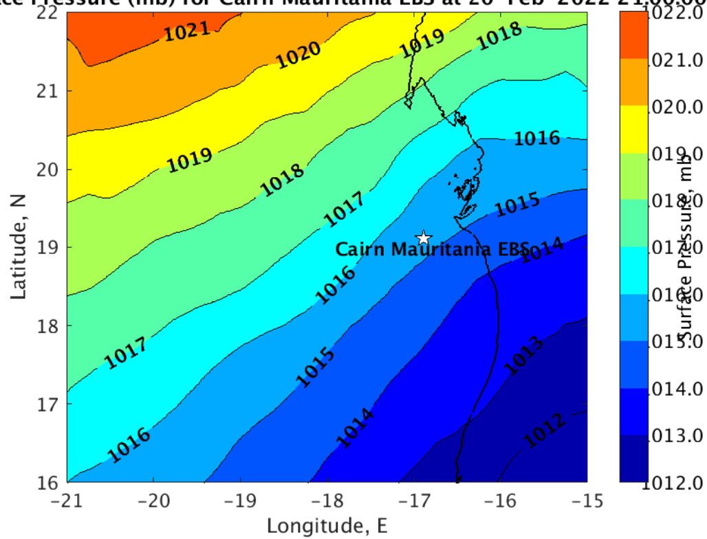
Surface Pressure (mb) for Cairn Mauritania EBS at 20-Feb-2022 21:00:00
