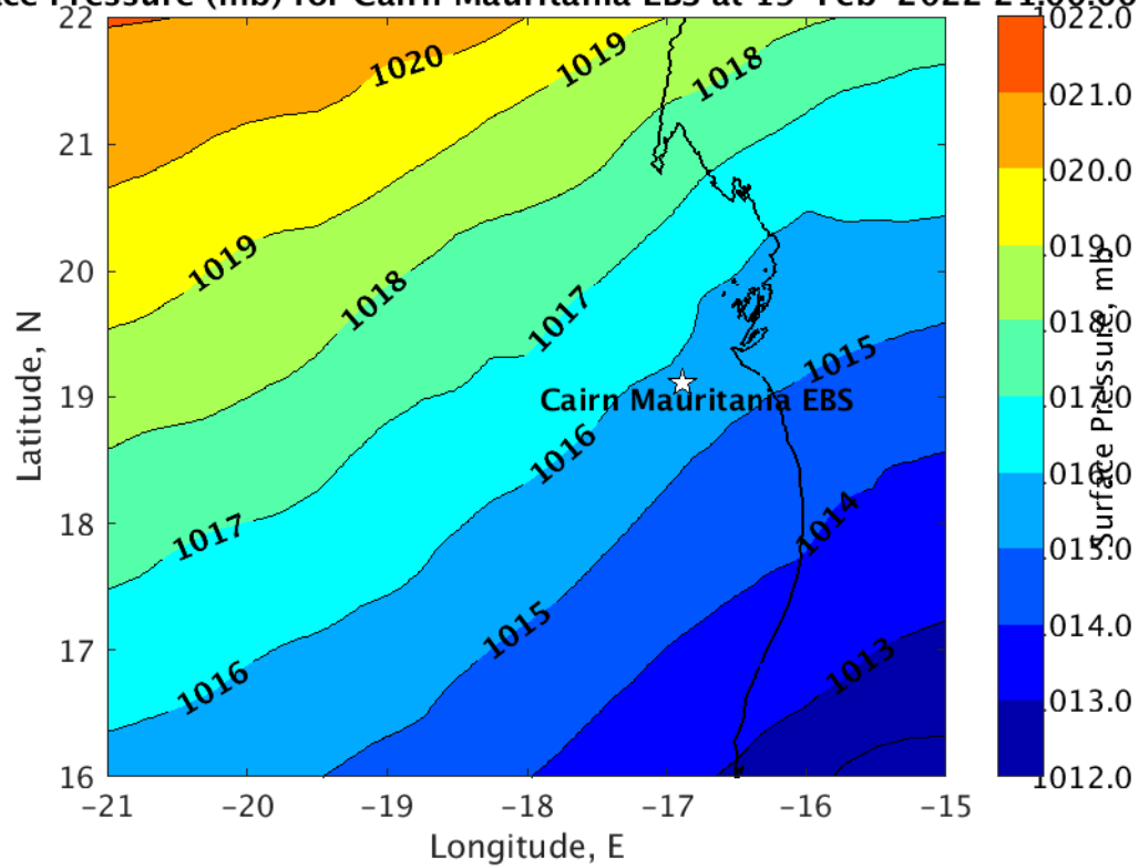
Surface Pressure (mb) for Cairn Mauritania EBS at 19-Feb-2022 21:00:00
