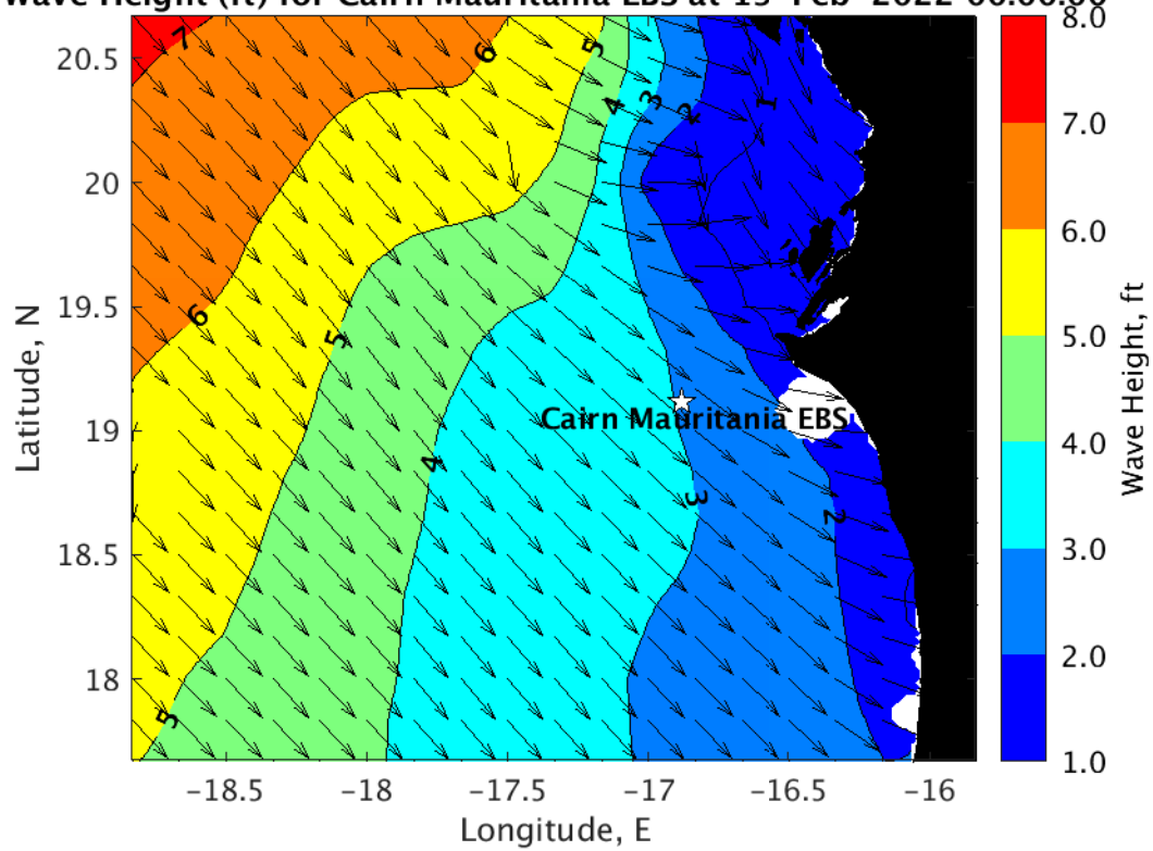
Wave Height (ft) for Cairn Mauritania EBS at 19-Feb-2022 00:00:00
