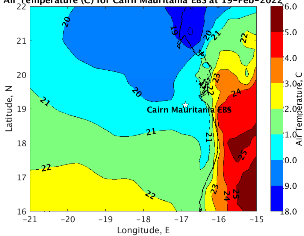
Air Temperature (C) for Cairn Mauritania EBS at 19-Feb-2022
