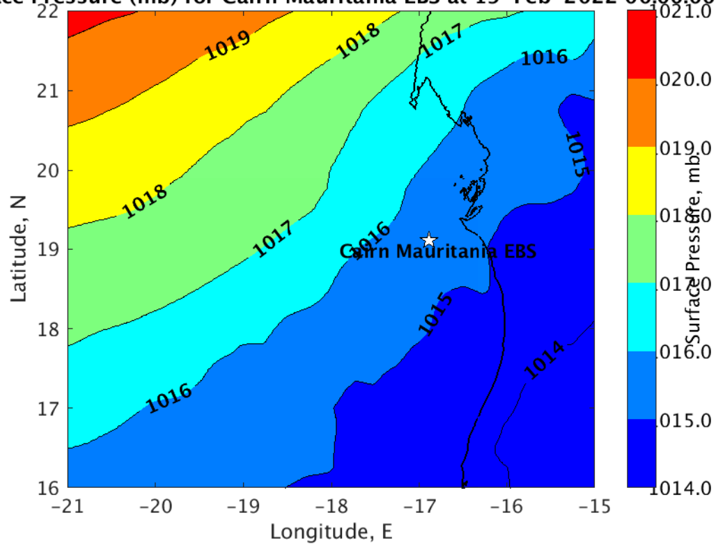
Surface Pressure (mb) for Cairn Mauritania EBS at 19-Feb-2022 00:00:00
