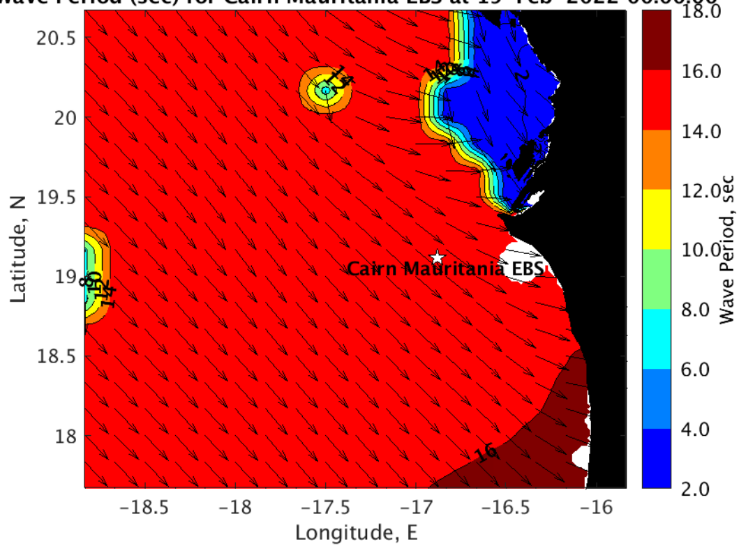
Wave Period (sec) for Cairn Mauritania EBS at 19-Feb-2022 00:00:00
