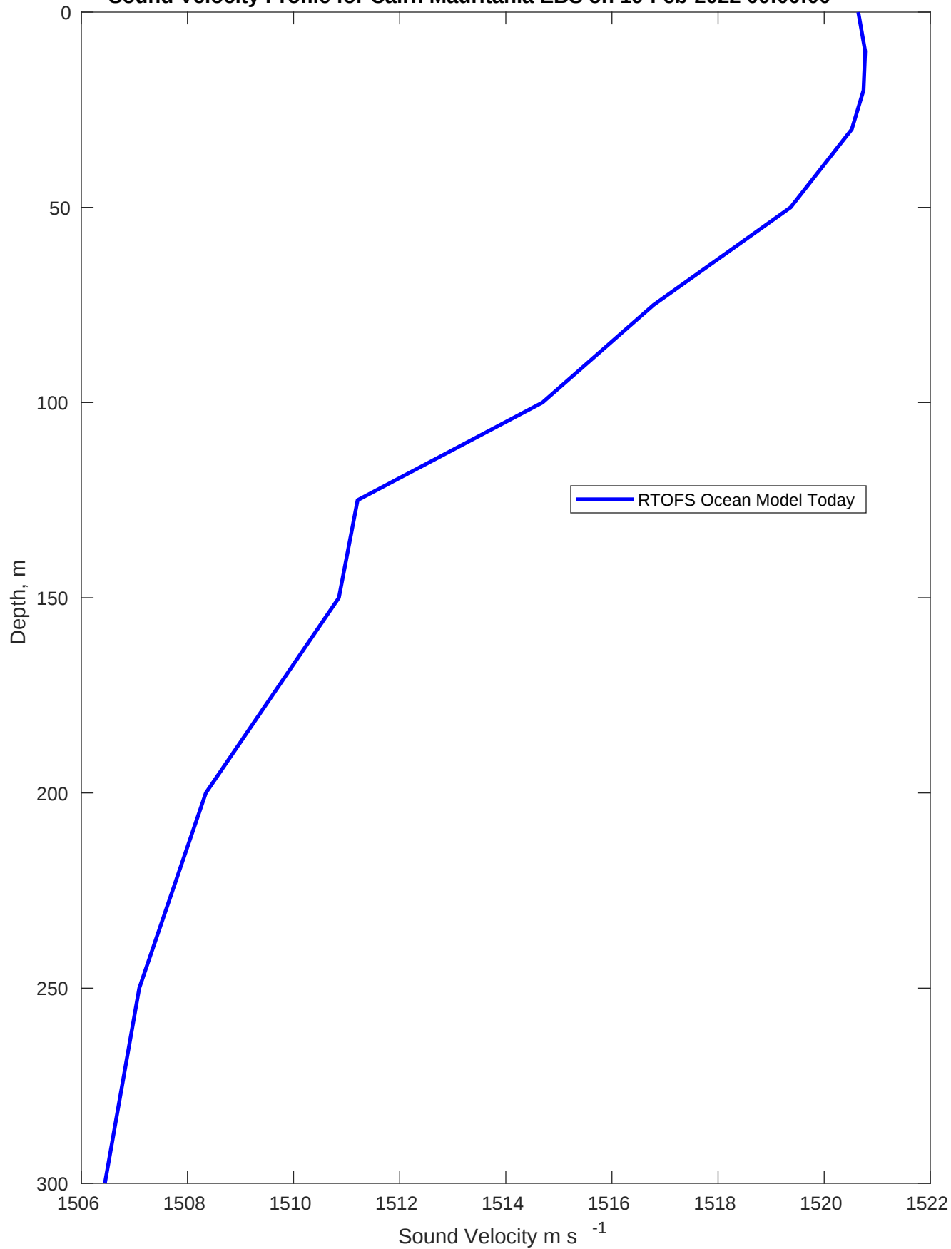
Sound Velocity Profile for Cairn Mauritania EBS on 19-Feb-2022 00:00:00
