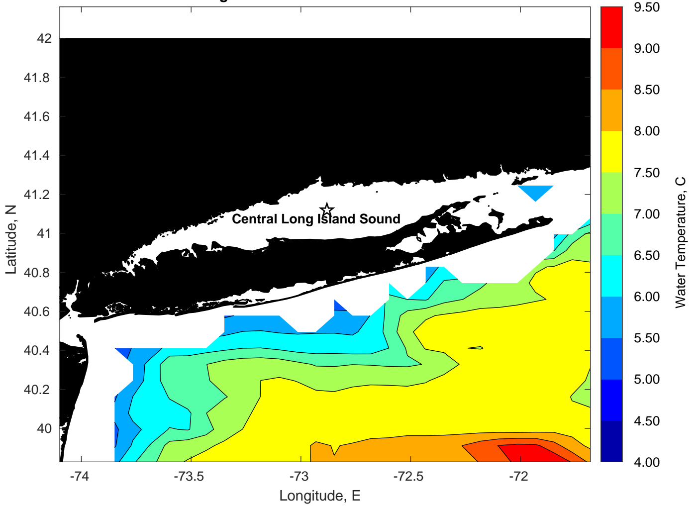
SST for Central Long Island Sound at 30-Jan-2024 00:00:00
