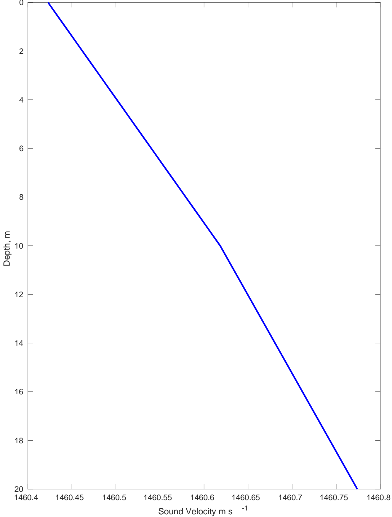
Sound Velocity Profile for Central Long Island Sound on 30-Jan-2024 00:00:00
