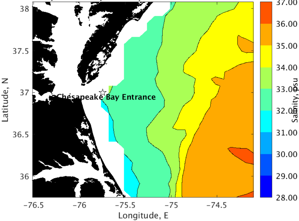
Surface Salinity for Chesapeake Bay Entrance at 08-Nov-2021 00:00:00
