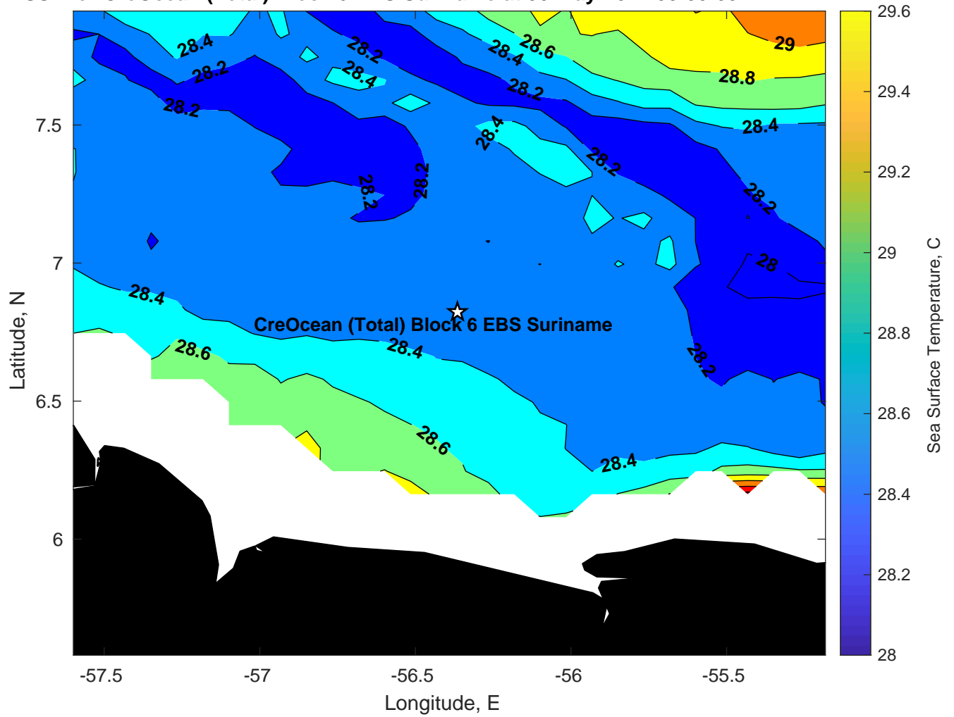
SST for CreOcean (Total) Block 6 EBS Suriname at 30-May-2024 00:00:00
