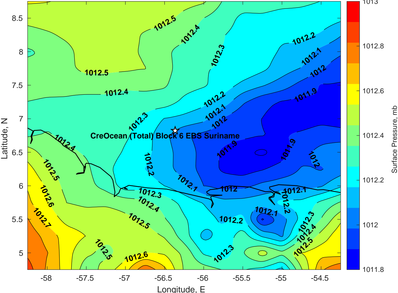
Surface Pressure (mb) for CreOcean (Total) Block 6 EBS Suriname at 31-May-2024 06:00:00
