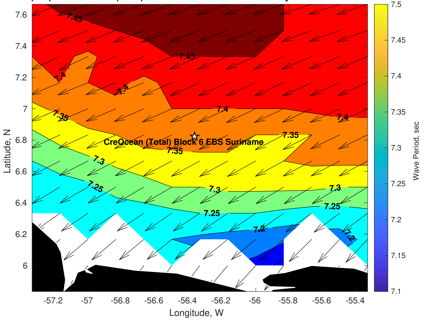
Wave Period (sec) for CreOcean (Total) Block 6 EBS Suriname at 31-May-2024 12:00:00
