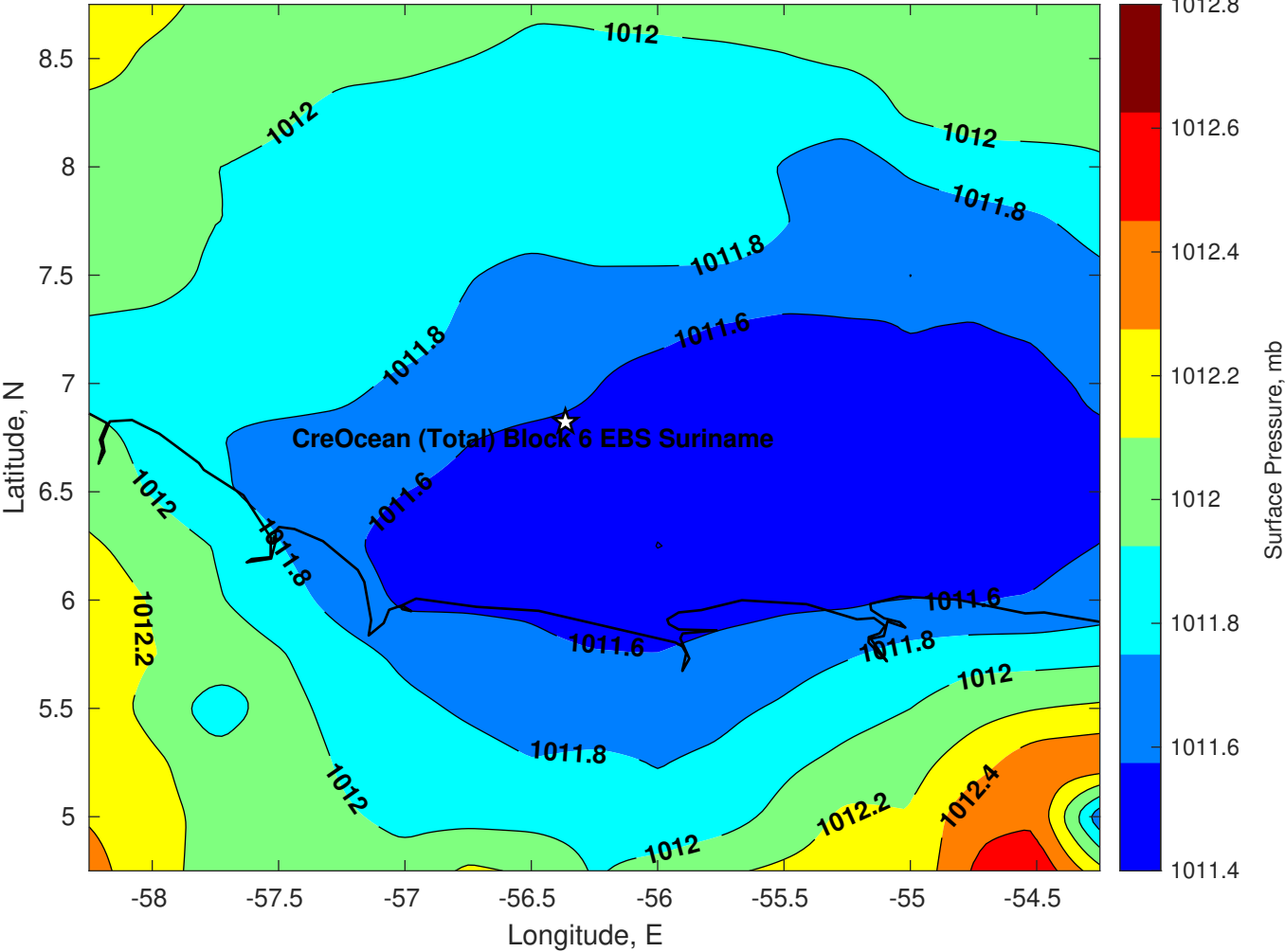
Surface Pressure (mb) for CreOcean (Total) Block 6 EBS Suriname at 01-Jun-2024 06:00:00
