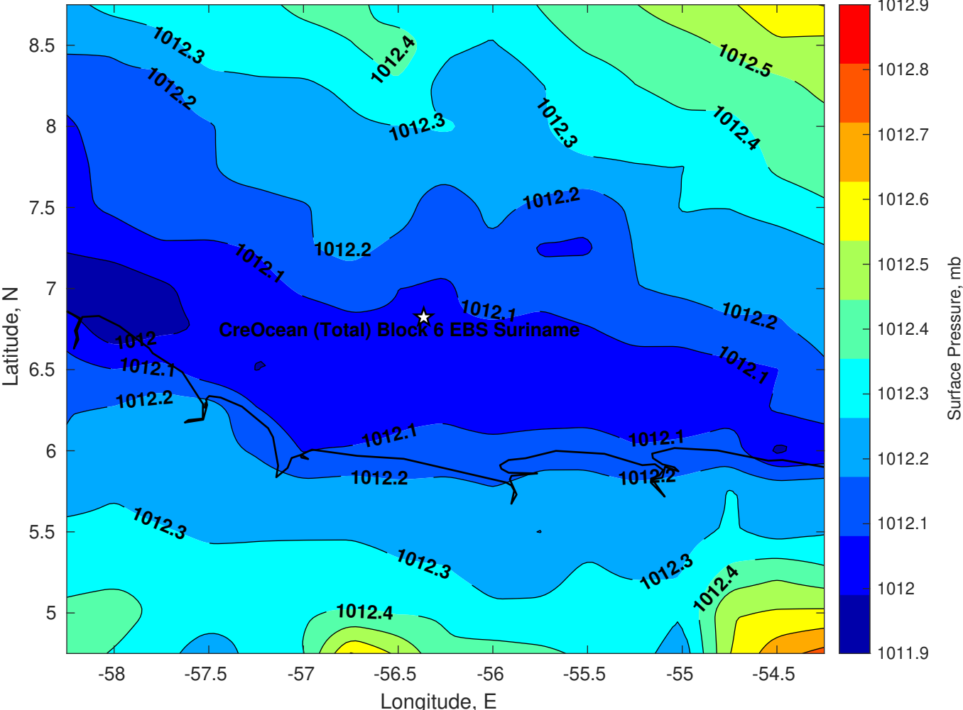
Surface Pressure (mb) for CreOcean (Total) Block 6 EBS Suriname at 02-Jun-2024 06:00:00
