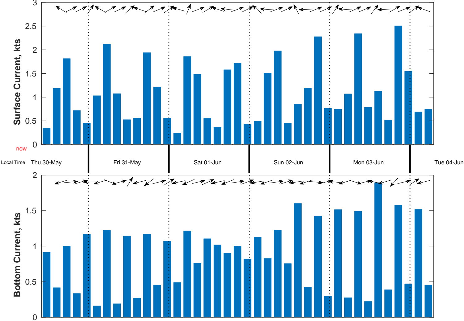
Surface Current Forecast for CreOcean (Total) Block 6 EBS Suriname from 31-May-2024 03:00:00 to 05-Jun-2024 00:00:00
