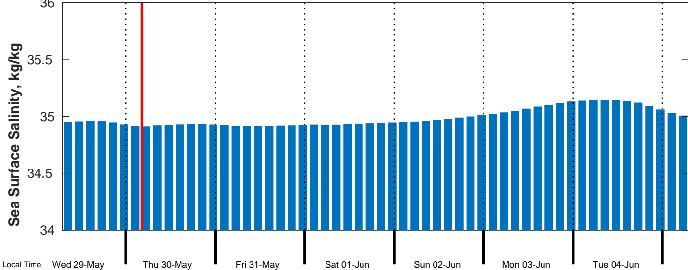
Sea Surface Salinity Forecast for CreOcean (Total) Block 6 EBS Suriname from 30-May-2024 00:00:00 to 06-Jun-2024 00:00:00
